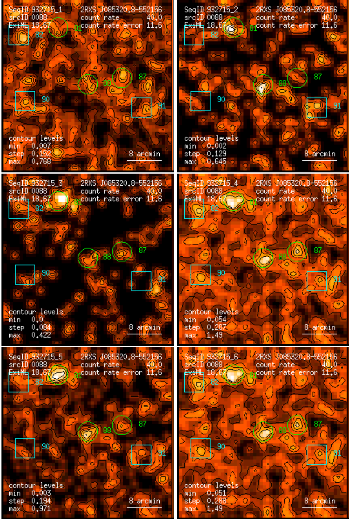
Figure 88: RASS 932715: detection 0088: band rate images, Gaussian filter: (1) PSPC channels 11 – 41, (2) 52 – 90, (3) 91 – 201, (4) 11 – 235, (5) 52 – 201, (6) 11 – 201. Broad band rates in counts/ks. Band rate contour levels in counts/ks/arcmin 2 .
