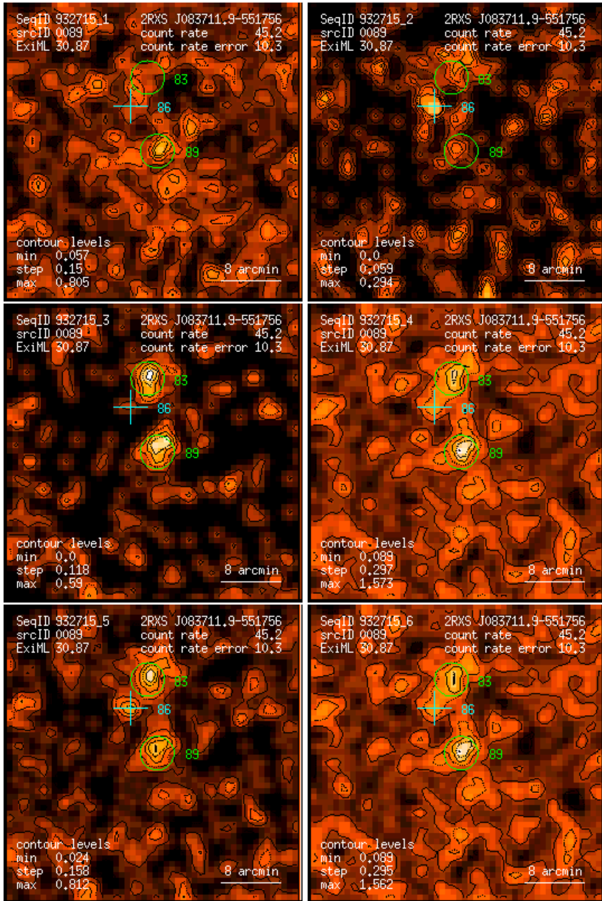
Figure 89: RASS 932715: detection 0089: band rate images, Gaussian filter: (1) PSPC channels 11 – 41, (2) 52 – 90, (3) 91 – 201, (4) 11 – 235, (5) 52 – 201, (6) 11 – 201. Broad band rates in counts/ks. Band rate contour levels in counts/ks/arcmin 2 .
