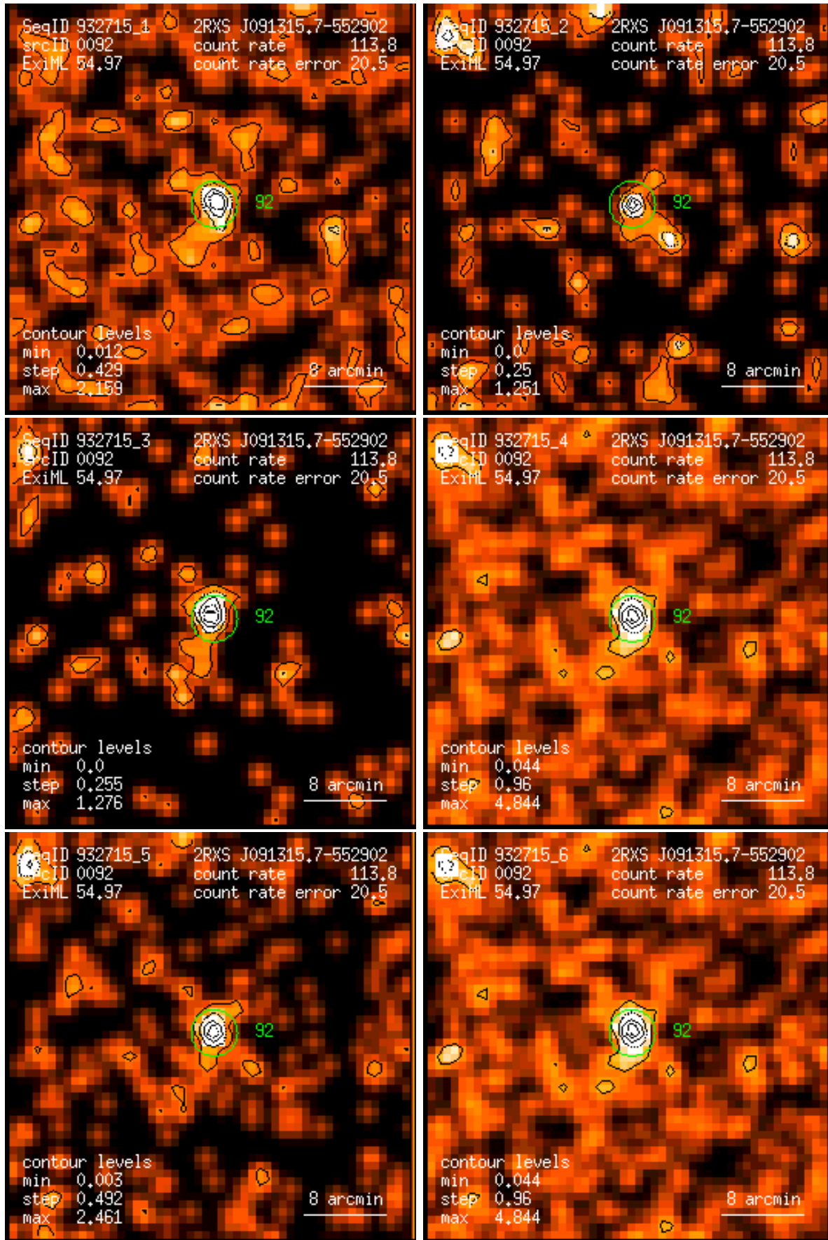
Figure 92: RASS 932715: detection 0092: band rate images, Gaussian filter: (1) PSPC channels 11 – 41, (2) 52 – 90, (3) 91 – 201, (4) 11 – 235, (5) 52 – 201, (6) 11 – 201. Broad band rates in counts/ks. Band rate contour levels in counts/ks/arcmin 2 .
