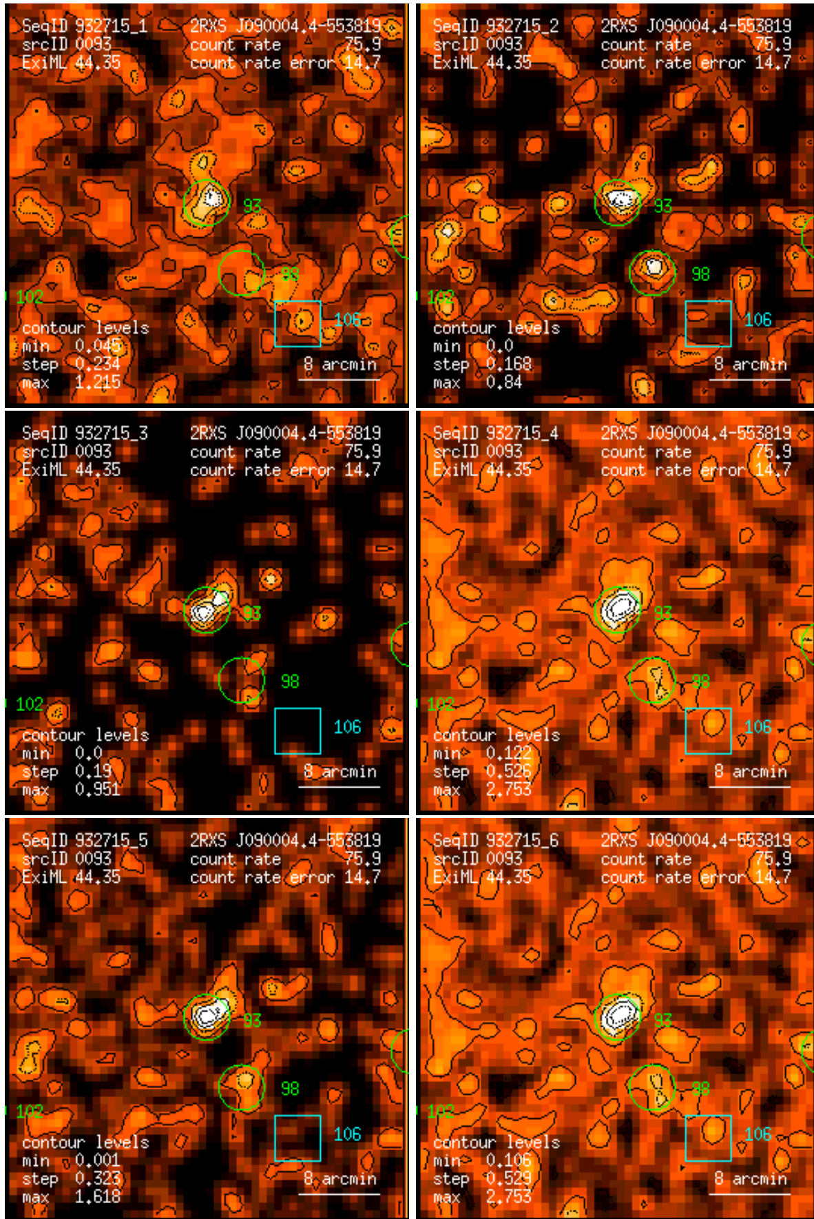
Figure 93: RASS 932715: detection 0093: band rate images, Gaussian filter: (1) PSPC channels 11 – 41, (2) 52 – 90, (3) 91 – 201, (4) 11 – 235, (5) 52 – 201, (6) 11 – 201. Broad band rates in counts/ks. Band rate contour levels in counts/ks/arcmin 2 .
