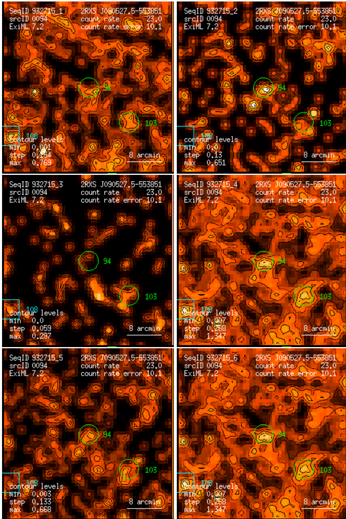
Figure 94: RASS 932715: detection 0094: band rate images, Gaussian filter: (1) PSPC channels 11 – 41, (2) 52 – 90, (3) 91 – 201, (4) 11 – 235, (5) 52 – 201, (6) 11 – 201. Broad band rates in counts/ks. Band rate contour levels in counts/ks/arcmin 2 .
