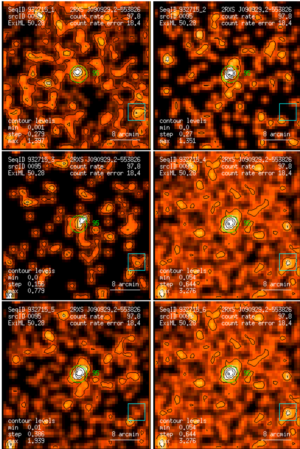
Figure 95: RASS 932715: detection 0095: band rate images, Gaussian filter: (1) PSPC channels 11 – 41, (2) 52 – 90, (3) 91 – 201, (4) 11 – 235, (5) 52 – 201, (6) 11 – 201. Broad band rates in counts/ks. Band rate contour levels in counts/ks/arcmin 2 .
