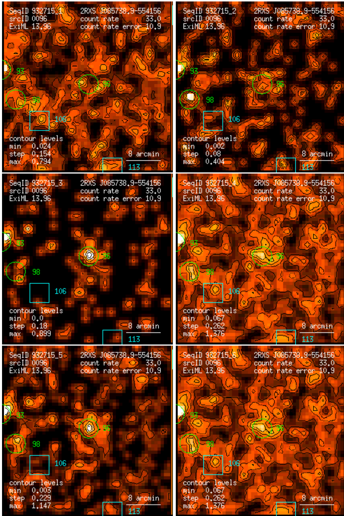
Figure 96: RASS 932715: detection 0096: band rate images, Gaussian filter: (1) PSPC channels 11 – 41, (2) 52 – 90, (3) 91 – 201, (4) 11 – 235, (5) 52 – 201, (6) 11 – 201. Broad band rates in counts/ks. Band rate contour levels in counts/ks/arcmin 2 .
