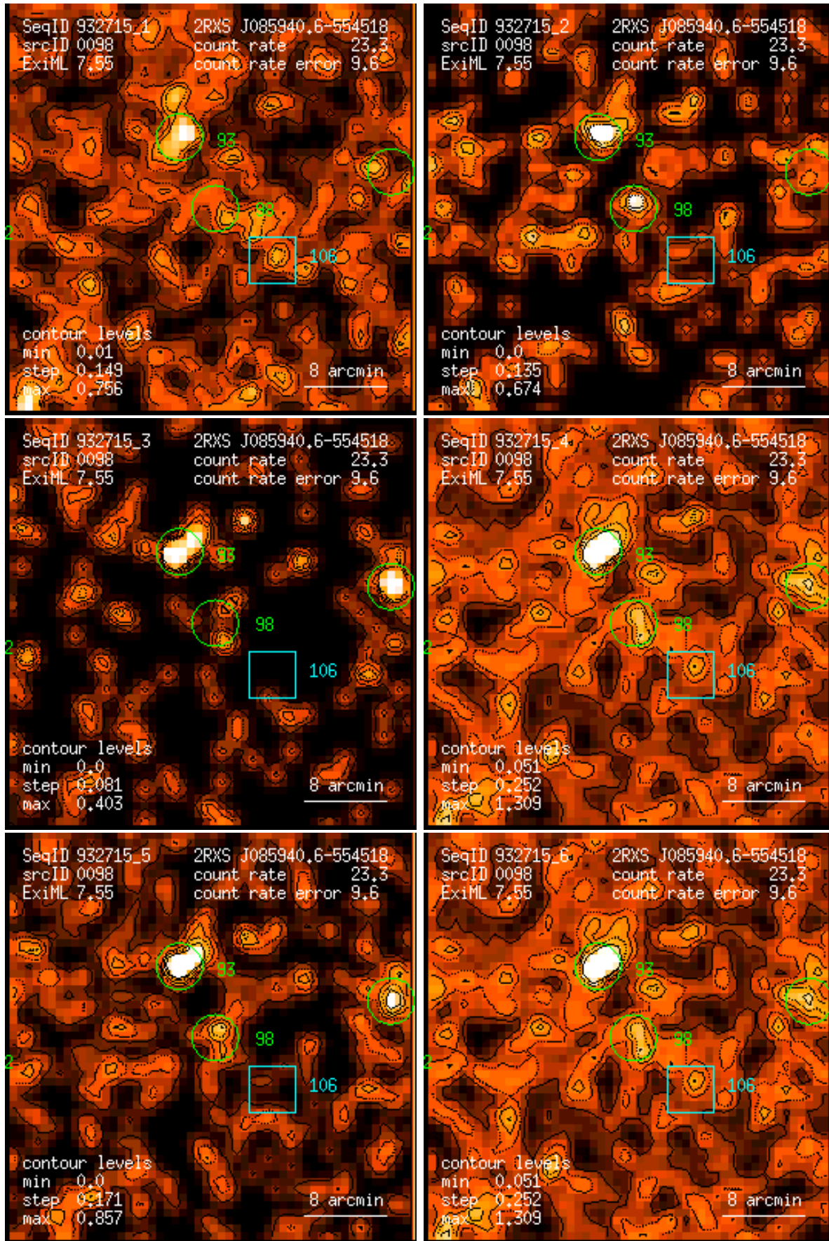
Figure 98: RASS 932715: detection 0098: band rate images, Gaussian filter: (1) PSPC channels 11 – 41, (2) 52 – 90, (3) 91 – 201, (4) 11 – 235, (5) 52 – 201, (6) 11 – 201. Broad band rates in counts/ks. Band rate contour levels in counts/ks/arcmin 2 .
