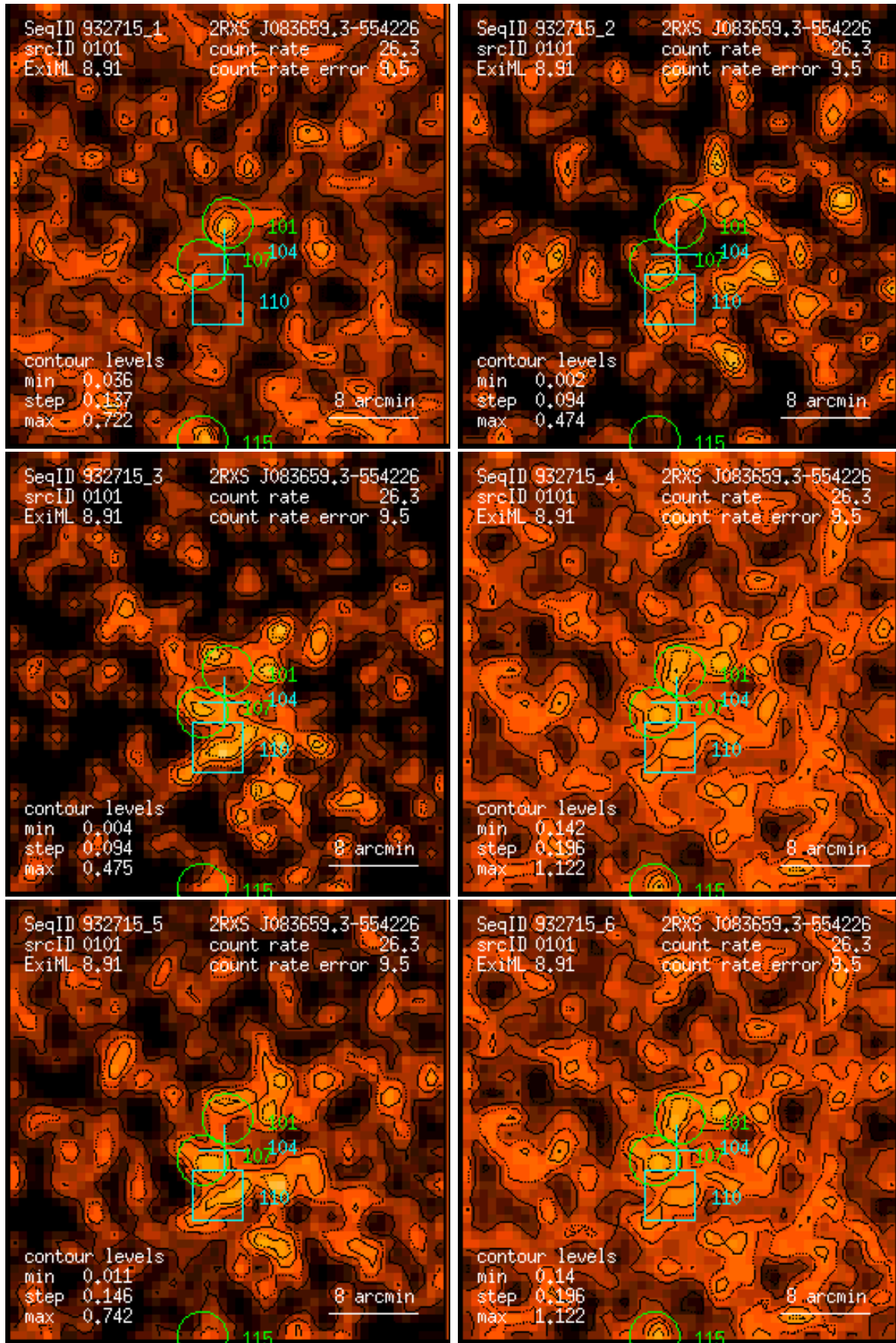
Figure 101: RASS 932715: detection 0101: band rate images, Gaussian filter: (1) PSPC channels 11 – 41, (2) 52 – 90, (3) 91 – 201, (4) 11 – 235, (5) 52 – 201, (6) 11 – 201. Broad band rates in counts/ks. Band rate contour levels in counts/ks/arcmin 2 .
