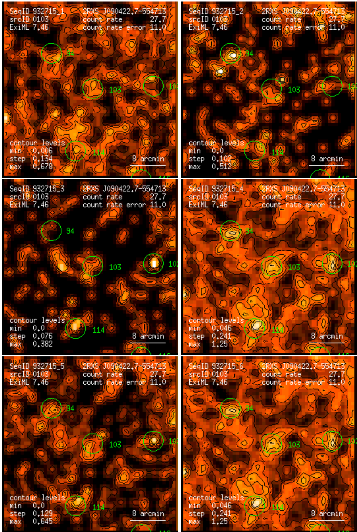
Figure 103: RASS 932715: detection 0103: band rate images, Gaussian filter: (1) PSPC channels 11 – 41, (2) 52 – 90, (3) 91 – 201, (4) 11 – 235, (5) 52 – 201, (6) 11 – 201. Broad band rates in counts/ks. Band rate contour levels in counts/ks/arcmin 2 .
