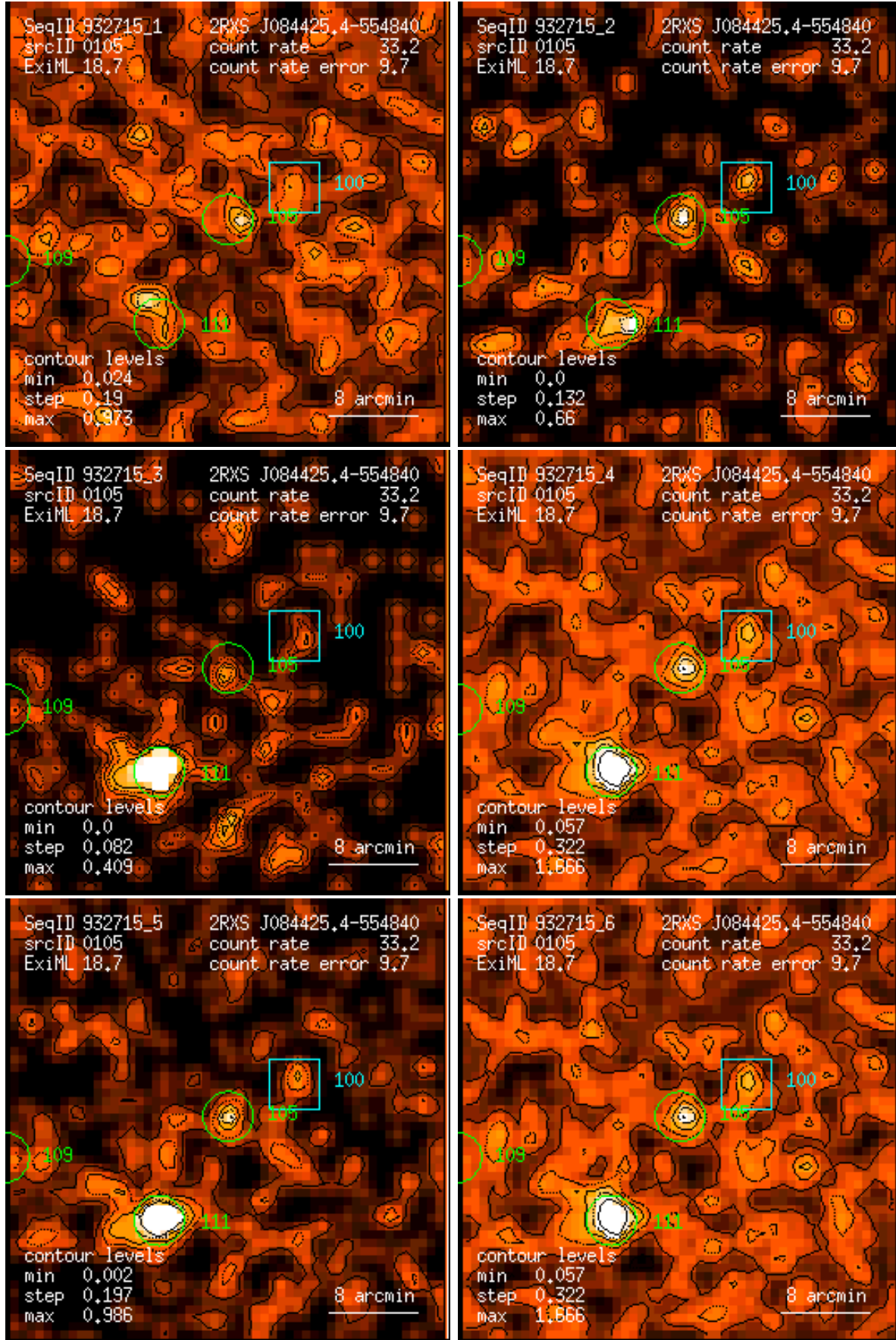
Figure 105: RASS 932715: detection 0105: band rate images, Gaussian filter: (1) PSPC channels 11 – 41, (2) 52 – 90, (3) 91 – 201, (4) 11 – 235, (5) 52 – 201, (6) 11 – 201. Broad band rates in counts/ks. Band rate contour levels in counts/ks/arcmin 2 .
