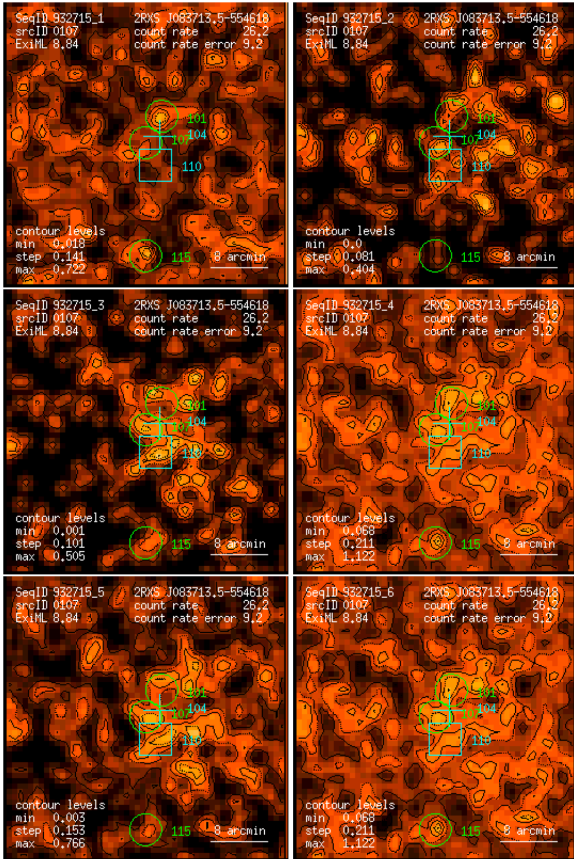
Figure 107: RASS 932715: detection 0107: band rate images, Gaussian filter: (1) PSPC channels 11 – 41, (2) 52 – 90, (3) 91 – 201, (4) 11 – 235, (5) 52 – 201, (6) 11 – 201. Broad band rates in counts/ks. Band rate contour levels in counts/ks/arcmin 2 .
