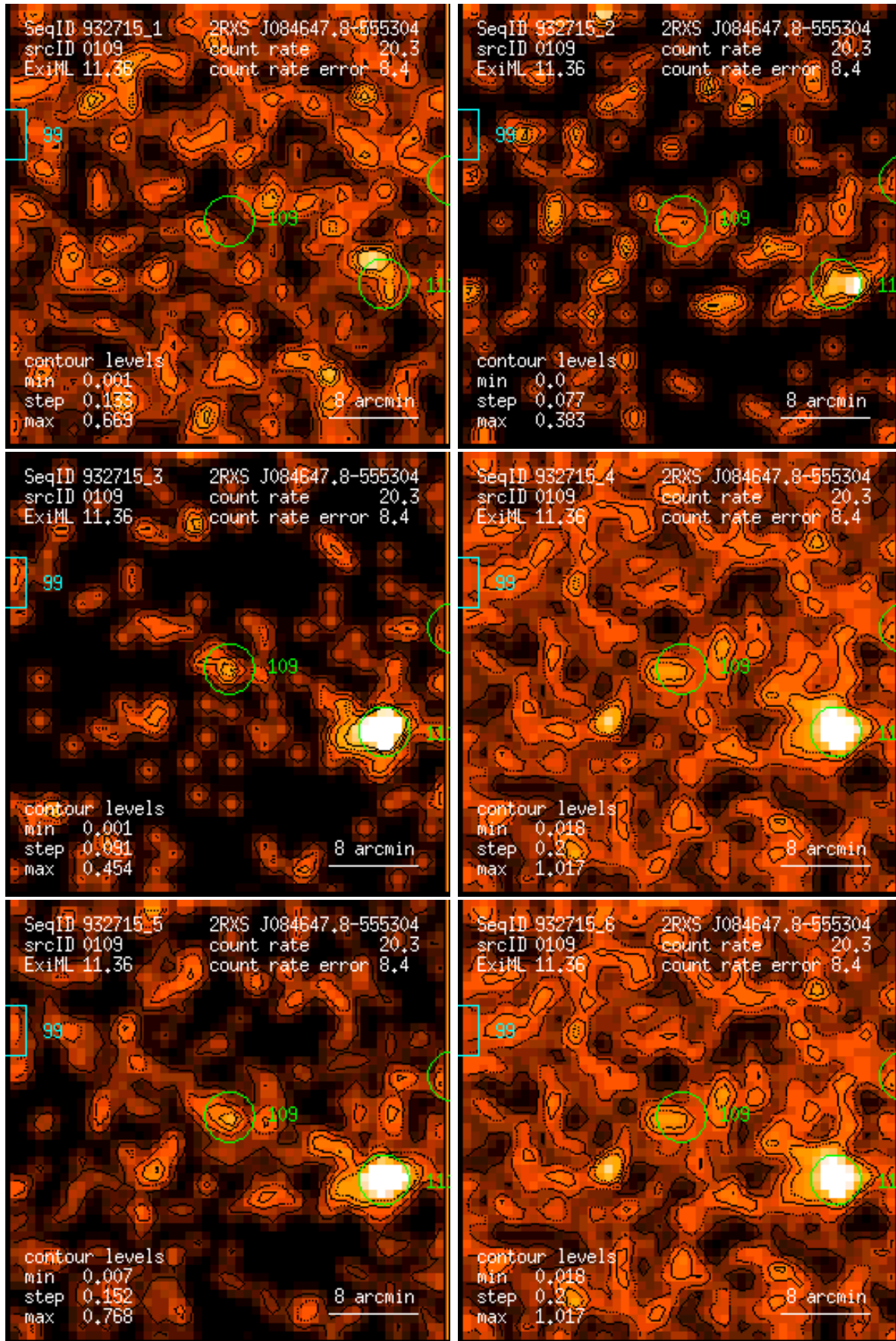
Figure 109: RASS 932715: detection 0109: band rate images, Gaussian filter: (1) PSPC channels 11 – 41, (2) 52 – 90, (3) 91 – 201, (4) 11 – 235, (5) 52 – 201, (6) 11 – 201. Broad band rates in counts/ks. Band rate contour levels in counts/ks/arcmin 2 .
