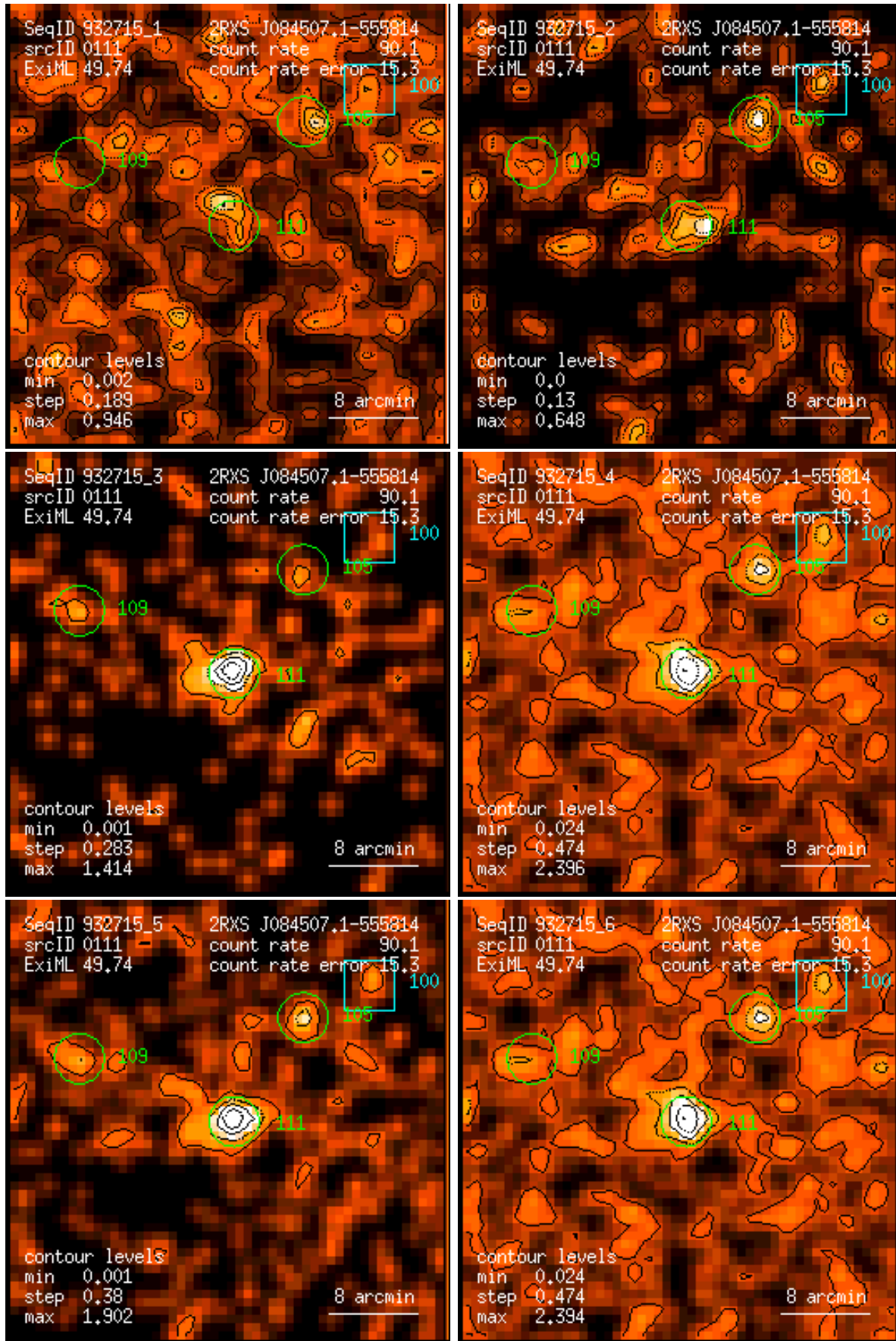
Figure 111: RASS 932715: detection 0111: band rate images, Gaussian filter: (1) PSPC channels 11 – 41, (2) 52 – 90, (3) 91 – 201, (4) 11 – 235, (5) 52 – 201, (6) 11 – 201. Broad band rates in counts/ks. Band rate contour levels in counts/ks/arcmin 2 .
