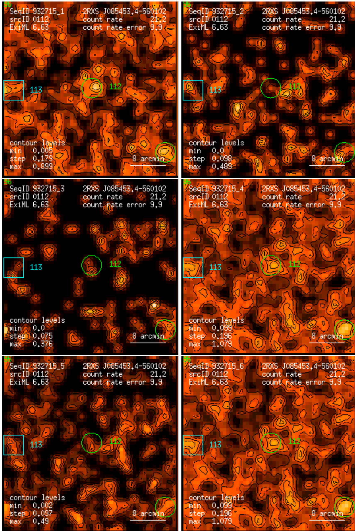
Figure 112: RASS 932715: detection 0112: band rate images, Gaussian filter: (1) PSPC channels 11 – 41, (2) 52 – 90, (3) 91 – 201, (4) 11 – 235, (5) 52 – 201, (6) 11 – 201. Broad band rates in counts/ks. Band rate contour levels in counts/ks/arcmin 2 .
