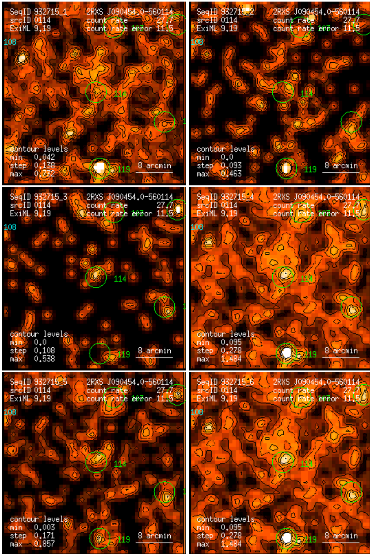
Figure 114: RASS 932715: detection 0114: band rate images, Gaussian filter: (1) PSPC channels 11 – 41, (2) 52 – 90, (3) 91 – 201, (4) 11 – 235, (5) 52 – 201, (6) 11 – 201. Broad band rates in counts/ks. Band rate contour levels in counts/ks/arcmin 2 .
