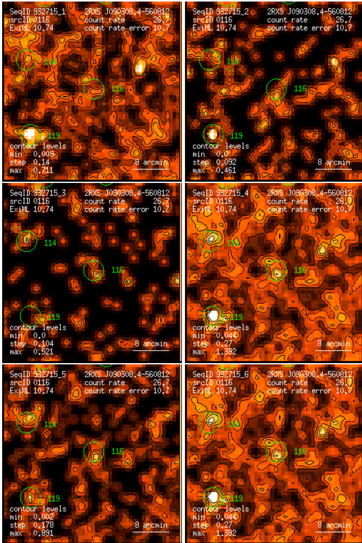
Figure 116: RASS 932715: detection 0116: band rate images, Gaussian filter: (1) PSPC channels 11 – 41, (2) 52 – 90, (3) 91 – 201, (4) 11 – 235, (5) 52 – 201, (6) 11 – 201. Broad band rates in counts/ks. Band rate contour levels in counts/ks/arcmin 2 .
