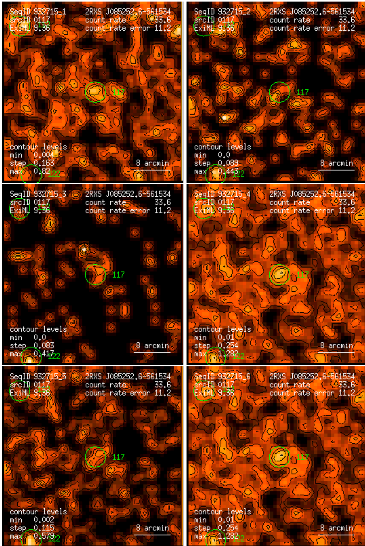
Figure 117: RASS 932715: detection 0117: band rate images, Gaussian filter: (1) PSPC channels 11 – 41, (2) 52 – 90, (3) 91 – 201, (4) 11 – 235, (5) 52 – 201, (6) 11 – 201. Broad band rates in counts/ks. Band rate contour levels in counts/ks/arcmin 2 .
