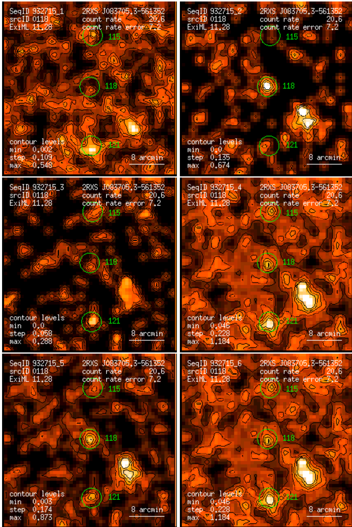
Figure 118: RASS 932715: detection 0118: band rate images, Gaussian filter: (1) PSPC channels 11 – 41, (2) 52 – 90, (3) 91 – 201, (4) 11 – 235, (5) 52 – 201, (6) 11 – 201. Broad band rates in counts/ks. Band rate contour levels in counts/ks/arcmin 2 .
