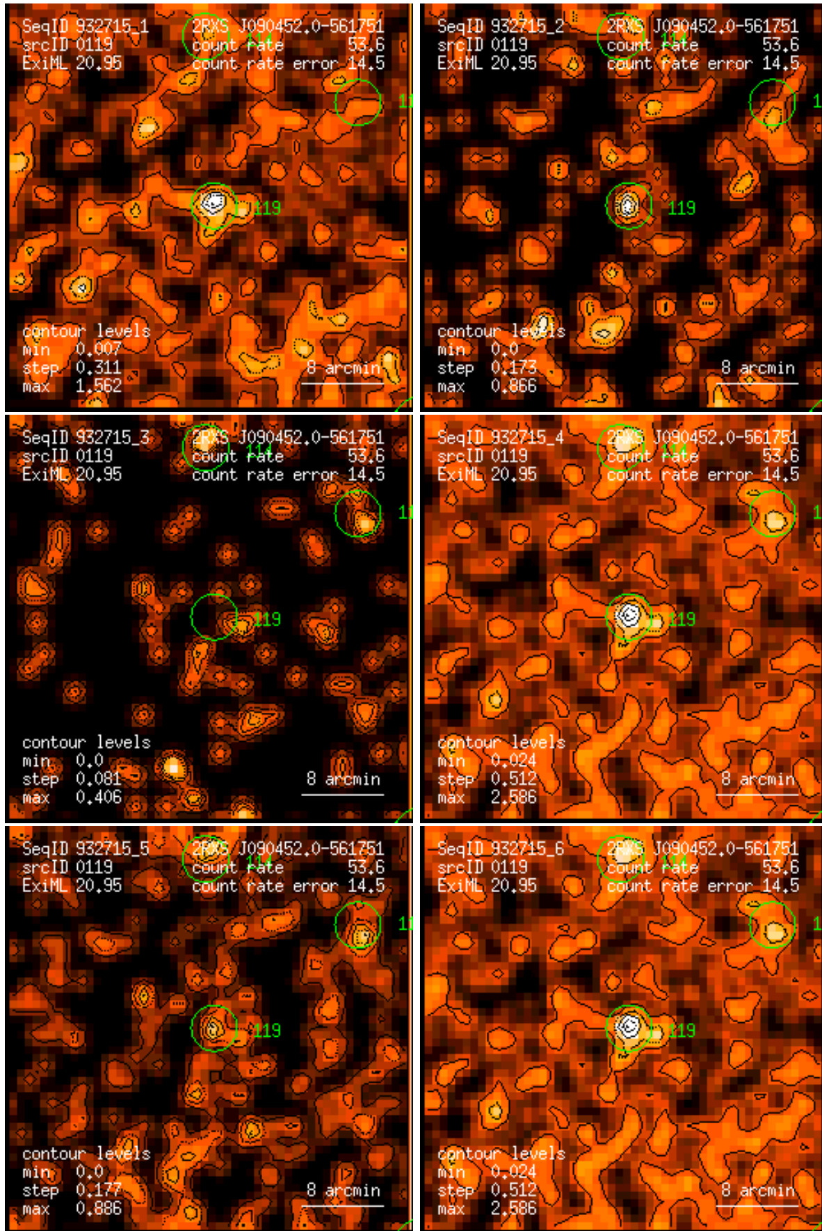
Figure 119: RASS 932715: detection 0119: band rate images, Gaussian filter: (1) PSPC channels 11 – 41, (2) 52 – 90, (3) 91 – 201, (4) 11 – 235, (5) 52 – 201, (6) 11 – 201. Broad band rates in counts/ks. Band rate contour levels in counts/ks/arcmin 2 .
