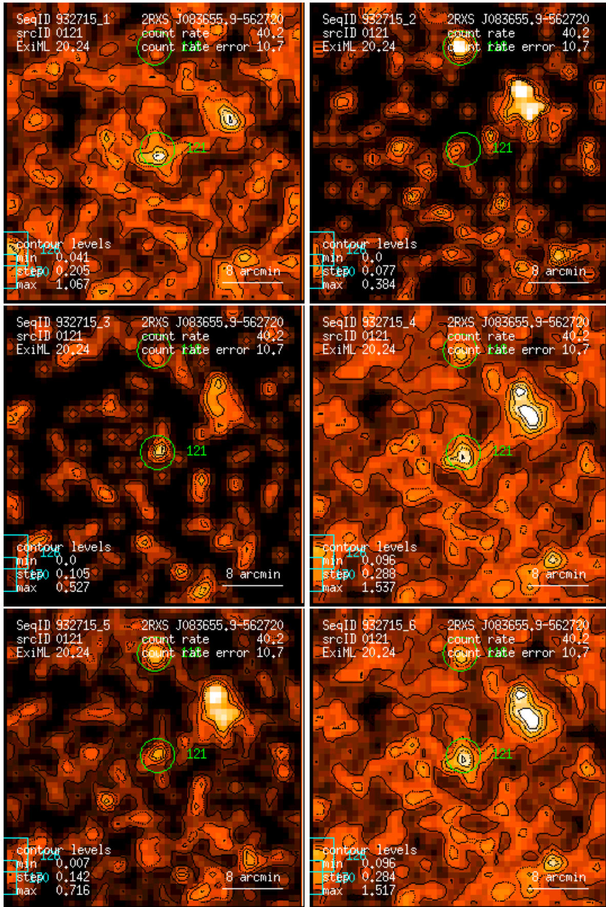
Figure 121: RASS 932715: detection 0121: band rate images, Gaussian filter: (1) PSPC channels 11 – 41, (2) 52 – 90, (3) 91 – 201, (4) 11 – 235, (5) 52 – 201, (6) 11 – 201. Broad band rates in counts/ks. Band rate contour levels in counts/ks/arcmin 2 .
