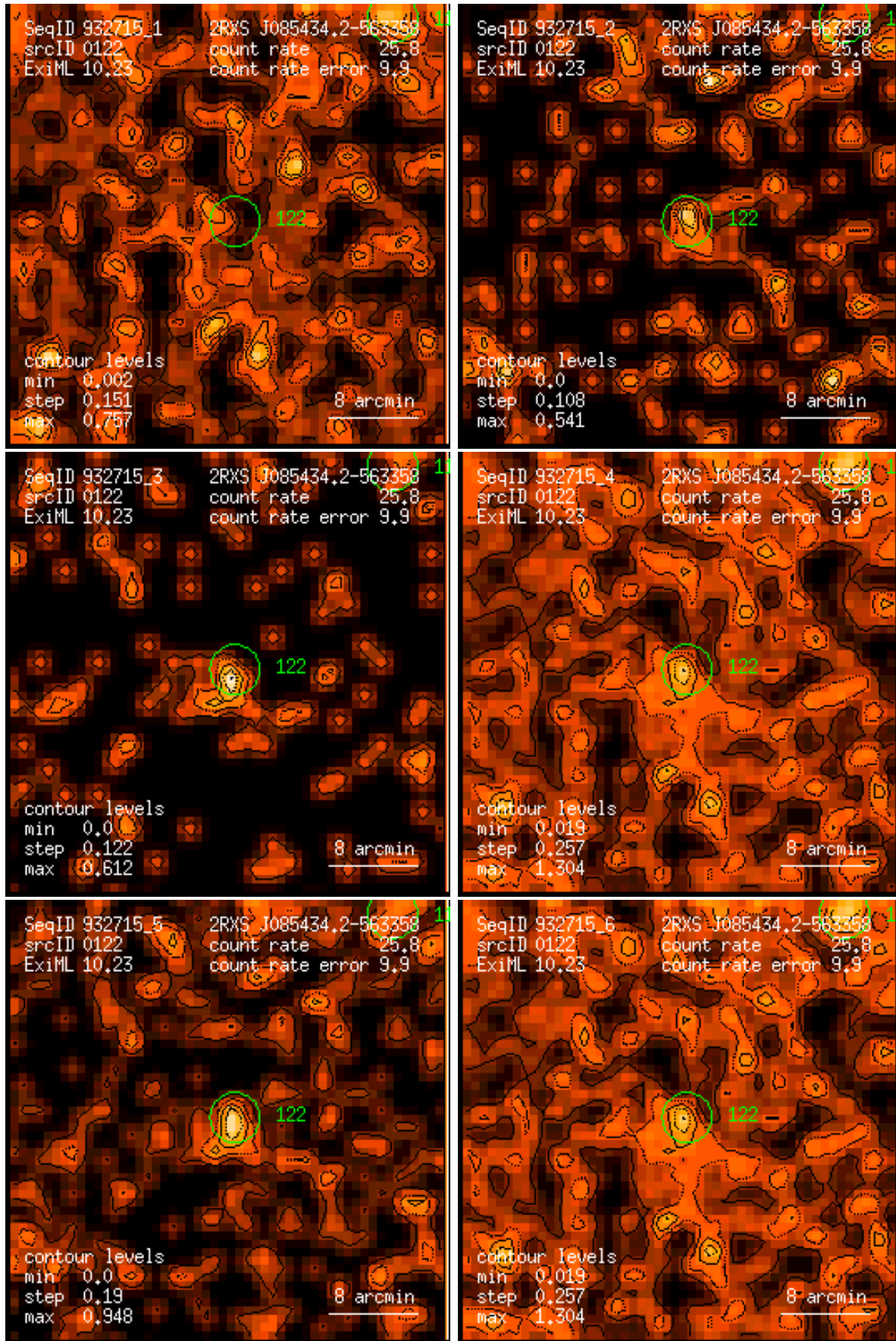
Figure 122: RASS 932715: detection 0122: band rate images, Gaussian filter: (1) PSPC channels 11 – 41, (2) 52 – 90, (3) 91 – 201, (4) 11 – 235, (5) 52 – 201, (6) 11 – 201. Broad band rates in counts/ks. Band rate contour levels in counts/ks/arcmin 2 .
