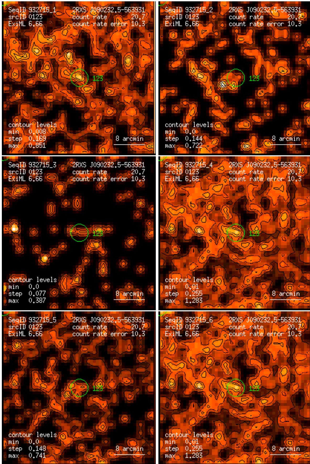
Figure 123: RASS 932715: detection 0123: band rate images, Gaussian filter: (1) PSPC channels 11 – 41, (2) 52 – 90, (3) 91 – 201, (4) 11 – 235, (5) 52 – 201, (6) 11 – 201. Broad band rates in counts/ks. Band rate contour levels in counts/ks/arcmin 2 .
