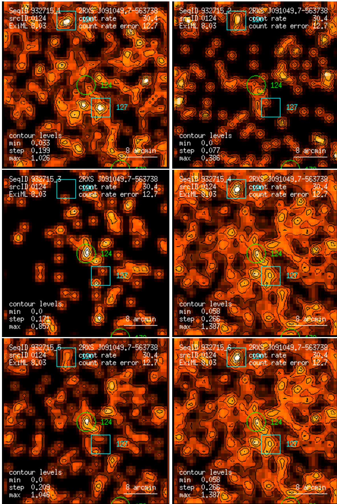
Figure 124: RASS 932715: detection 0124: band rate images, Gaussian filter: (1) PSPC channels 11 – 41, (2) 52 – 90, (3) 91 – 201, (4) 11 – 235, (5) 52 – 201, (6) 11 – 201. Broad band rates in counts/ks. Band rate contour levels in counts/ks/arcmin 2 .
