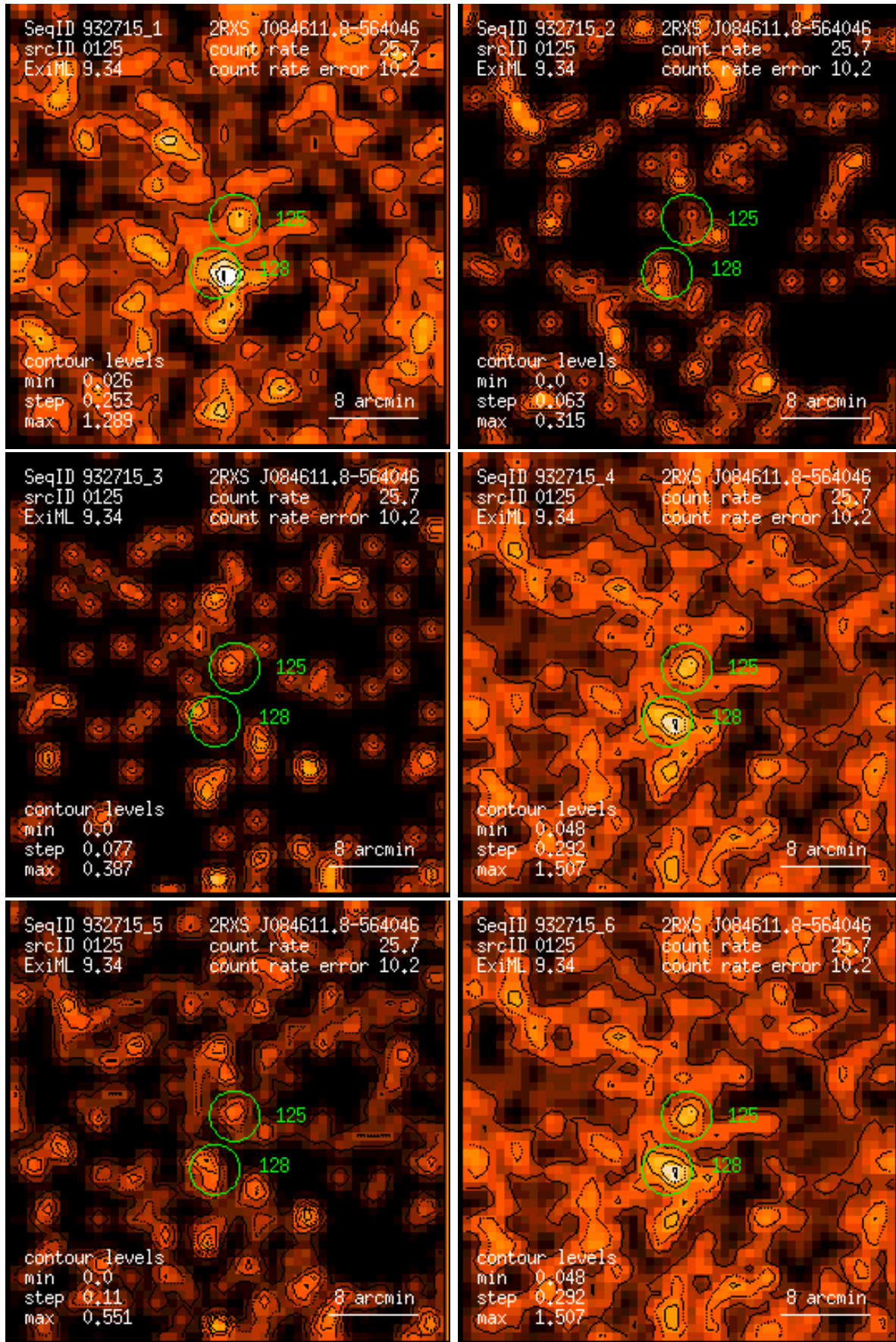
Figure 125: RASS 932715: detection 0125: band rate images, Gaussian filter: (1) PSPC channels 11 – 41, (2) 52 – 90, (3) 91 – 201, (4) 11 – 235, (5) 52 – 201, (6) 11 – 201. Broad band rates in counts/ks. Band rate contour levels in counts/ks/arcmin 2 .
