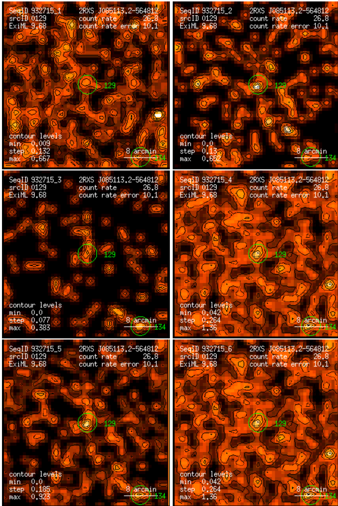
Figure 129: RASS 932715: detection 0129: band rate images, Gaussian filter: (1) PSPC channels 11 – 41, (2) 52 – 90, (3) 91 – 201, (4) 11 – 235, (5) 52 – 201, (6) 11 – 201. Broad band rates in counts/ks. Band rate contour levels in counts/ks/arcmin 2 .
