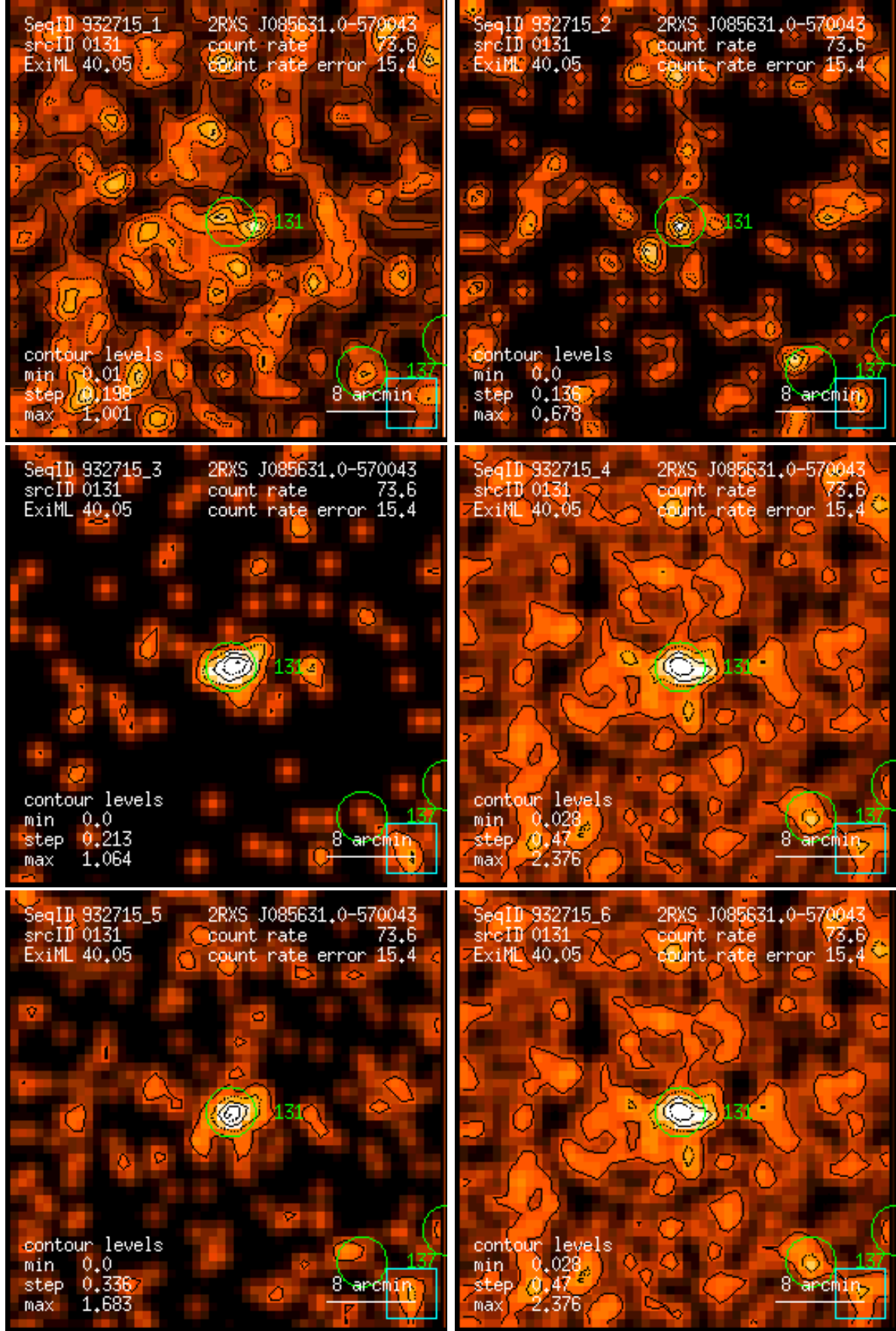
Figure 131: RASS 932715: detection 0131: band rate images, Gaussian filter: (1) PSPC channels 11 – 41, (2) 52 – 90, (3) 91 – 201, (4) 11 – 235, (5) 52 – 201, (6) 11 – 201. Broad band rates in counts/ks. Band rate contour levels in counts/ks/arcmin 2 .
