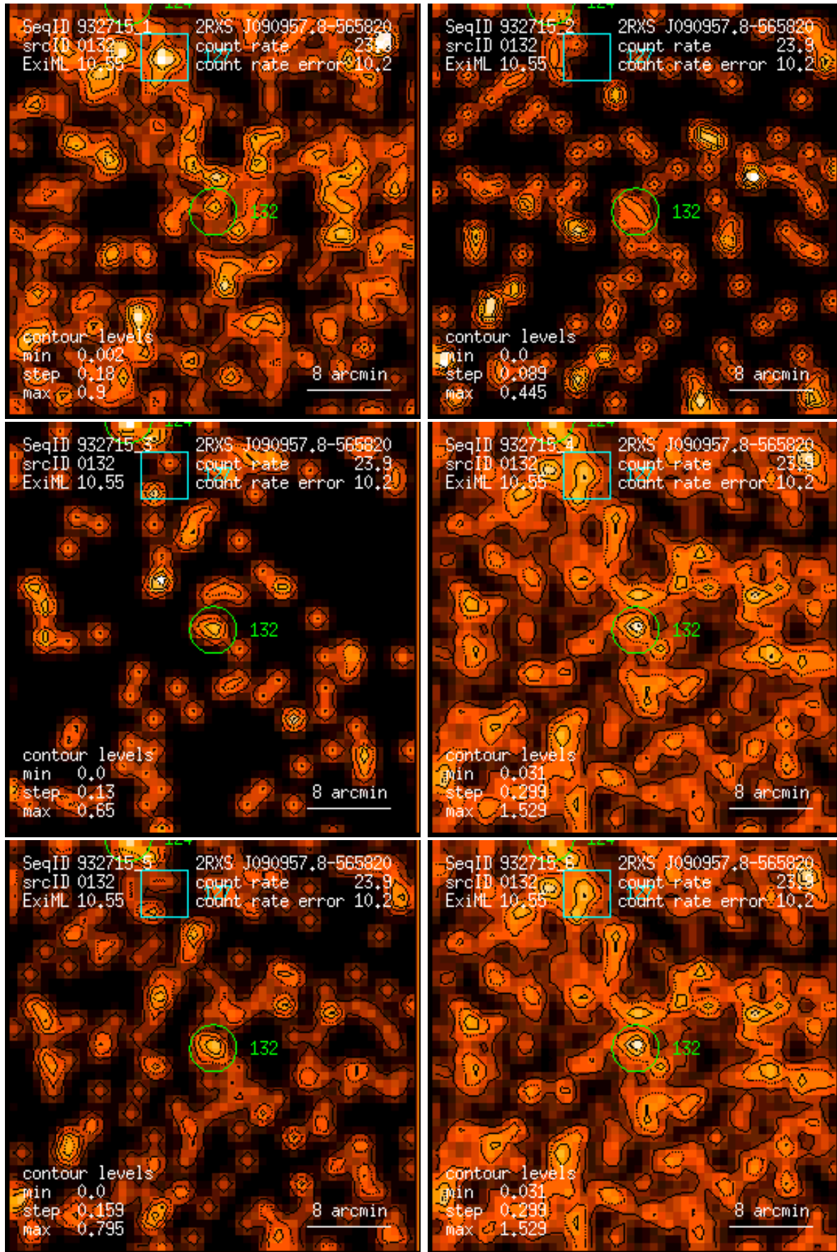
Figure 132: RASS 932715: detection 0132: band rate images, Gaussian filter: (1) PSPC channels 11 – 41, (2) 52 – 90, (3) 91 – 201, (4) 11 – 235, (5) 52 – 201, (6) 11 – 201. Broad band rates in counts/ks. Band rate contour levels in counts/ks/arcmin 2 .
