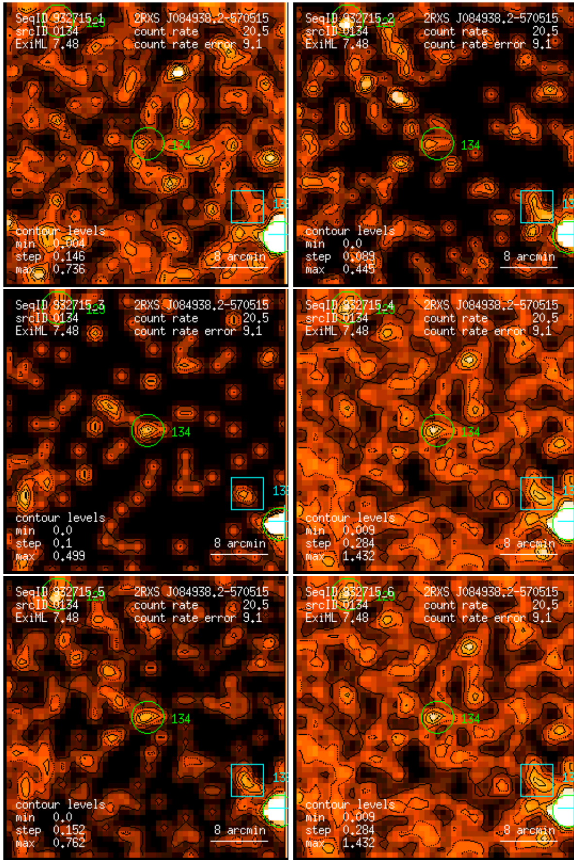
Figure 134: RASS 932715: detection 0134: band rate images, Gaussian filter: (1) PSPC channels 11 – 41, (2) 52 – 90, (3) 91 – 201, (4) 11 – 235, (5) 52 – 201, (6) 11 – 201. Broad band rates in counts/ks. Band rate contour levels in counts/ks/arcmin 2 .
