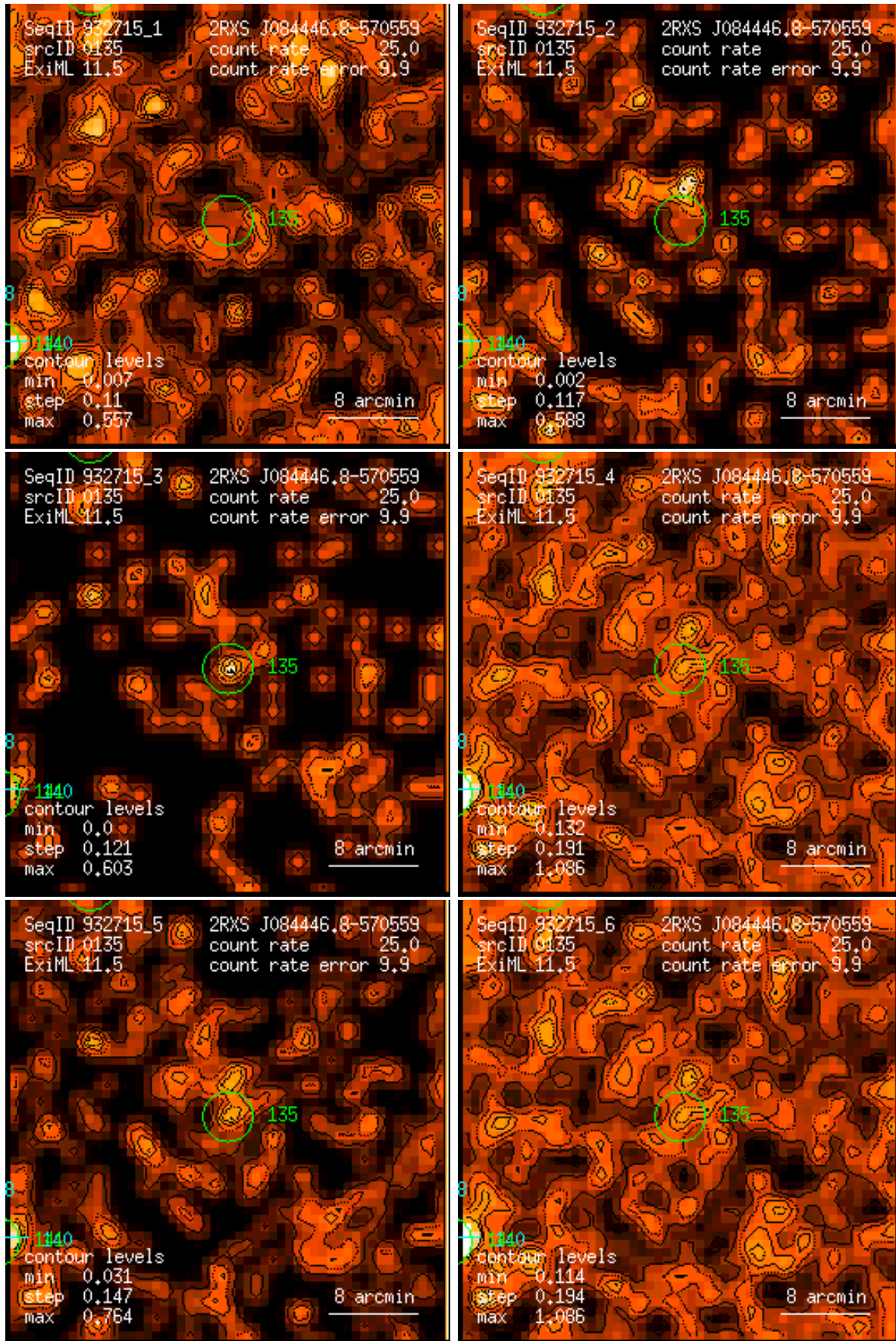
Figure 135: RASS 932715: detection 0135: band rate images, Gaussian filter: (1) PSPC channels 11 – 41, (2) 52 – 90, (3) 91 – 201, (4) 11 – 235, (5) 52 – 201, (6) 11 – 201. Broad band rates in counts/ks. Band rate contour levels in counts/ks/arcmin 2 .
