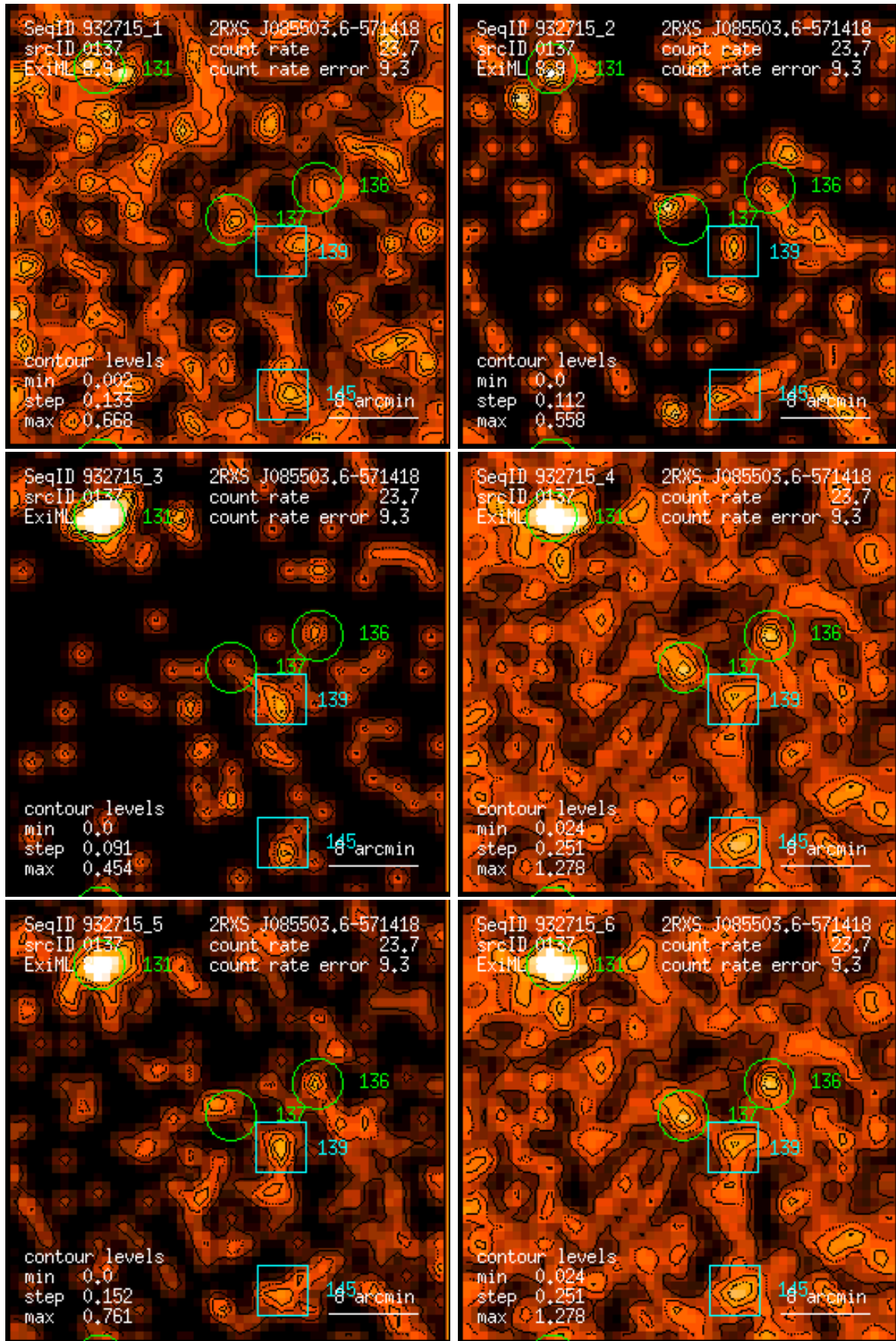
Figure 137: RASS 932715: detection 0137: band rate images, Gaussian filter: (1) PSPC channels 11 – 41, (2) 52 – 90, (3) 91 – 201, (4) 11 – 235, (5) 52 – 201, (6) 11 – 201. Broad band rates in counts/ks. Band rate contour levels in counts/ks/arcmin 2 .
