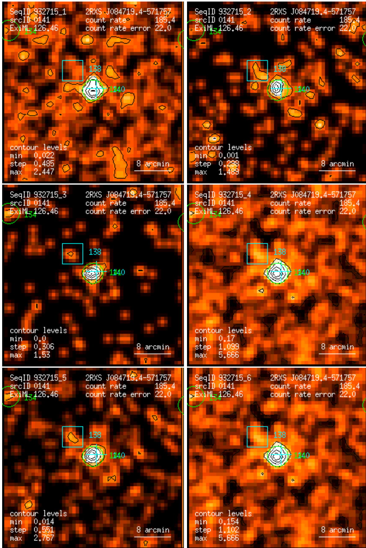
Figure 141: RASS 932715: detection 0141: band rate images, Gaussian filter: (1) PSPC channels 11 – 41, (2) 52 – 90, (3) 91 – 201, (4) 11 – 235, (5) 52 – 201, (6) 11 – 201. Broad band rates in counts/ks. Band rate contour levels in counts/ks/arcmin 2 .
