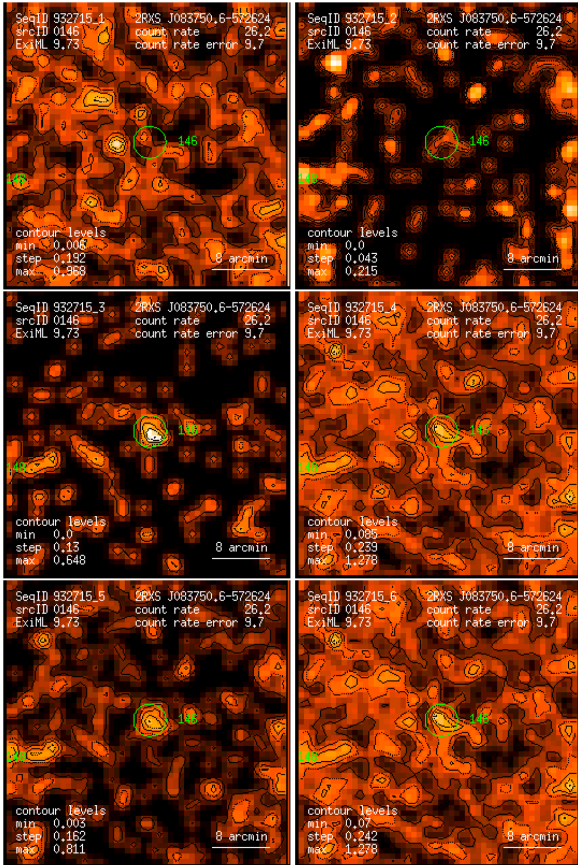
Figure 146: RASS 932715: detection 0146: band rate images, Gaussian filter: (1) PSPC channels 11 – 41, (2) 52 – 90, (3) 91 – 201, (4) 11 – 235, (5) 52 – 201, (6) 11 – 201. Broad band rates in counts/ks. Band rate contour levels in counts/ks/arcmin 2 .
