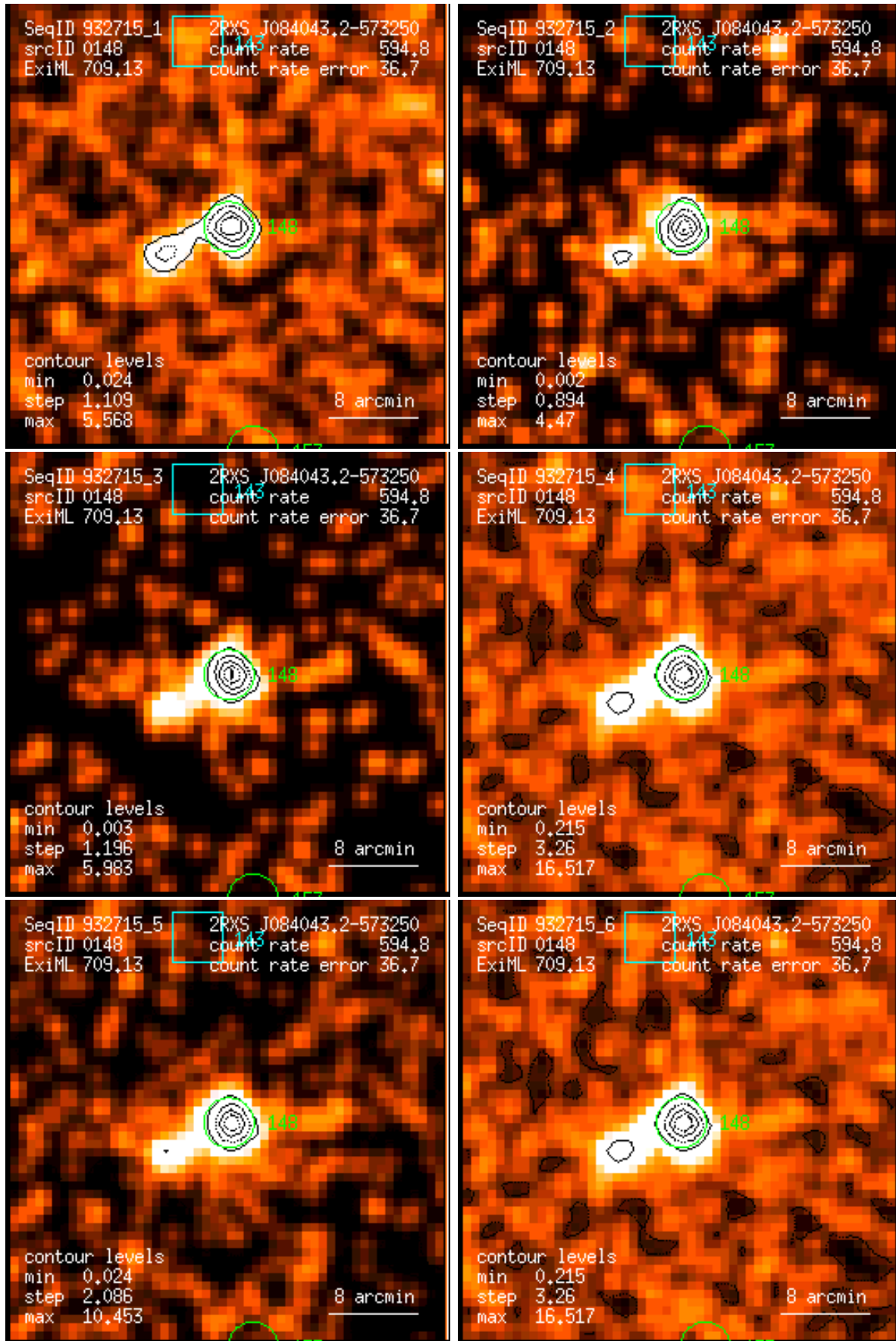
Figure 148: RASS 932715: detection 0148: band rate images, Gaussian filter: (1) PSPC channels 11 – 41, (2) 52 – 90, (3) 91 – 201, (4) 11 – 235, (5) 52 – 201, (6) 11 – 201. Broad band rates in counts/ks. Band rate contour levels in counts/ks/arcmin 2 .
