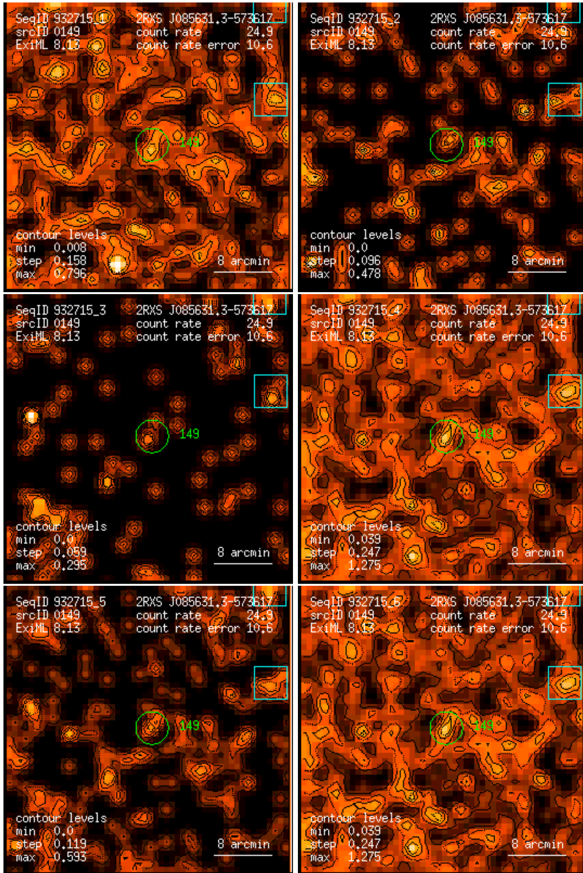
Figure 149: RASS 932715: detection 0149: band rate images, Gaussian filter: (1) PSPC channels 11 – 41, (2) 52 – 90, (3) 91 – 201, (4) 11 – 235, (5) 52 – 201, (6) 11 – 201. Broad band rates in counts/ks. Band rate contour levels in counts/ks/arcmin 2 .
