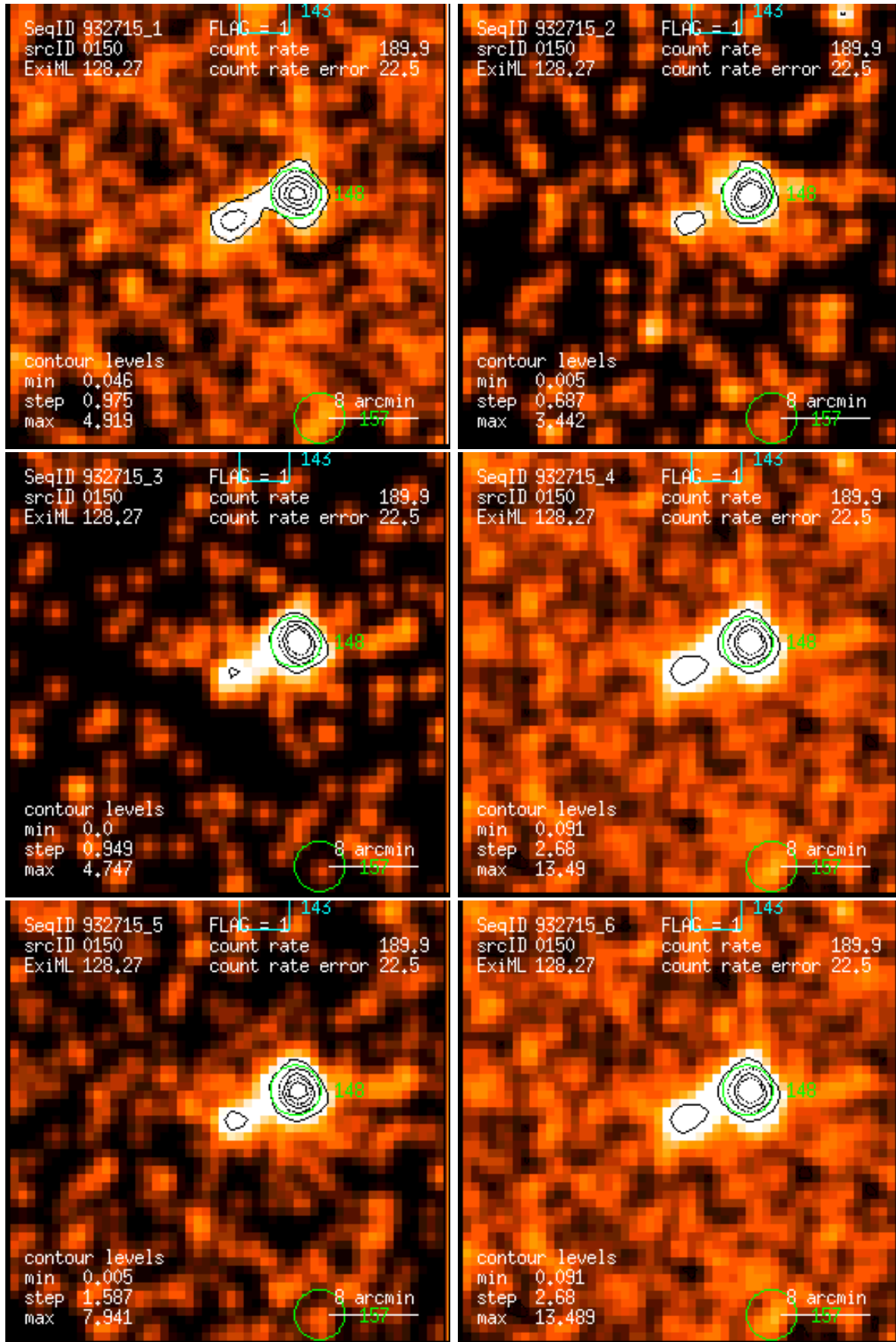
Figure 150: RASS 932715: detection 0150: band rate images, Gaussian filter: (1) PSPC channels 11 – 41, (2) 52 – 90, (3) 91 – 201, (4) 11 – 235, (5) 52 – 201, (6) 11 – 201. Broad band rates in counts/ks. Band rate contour levels in counts/ks/arcmin 2 .
