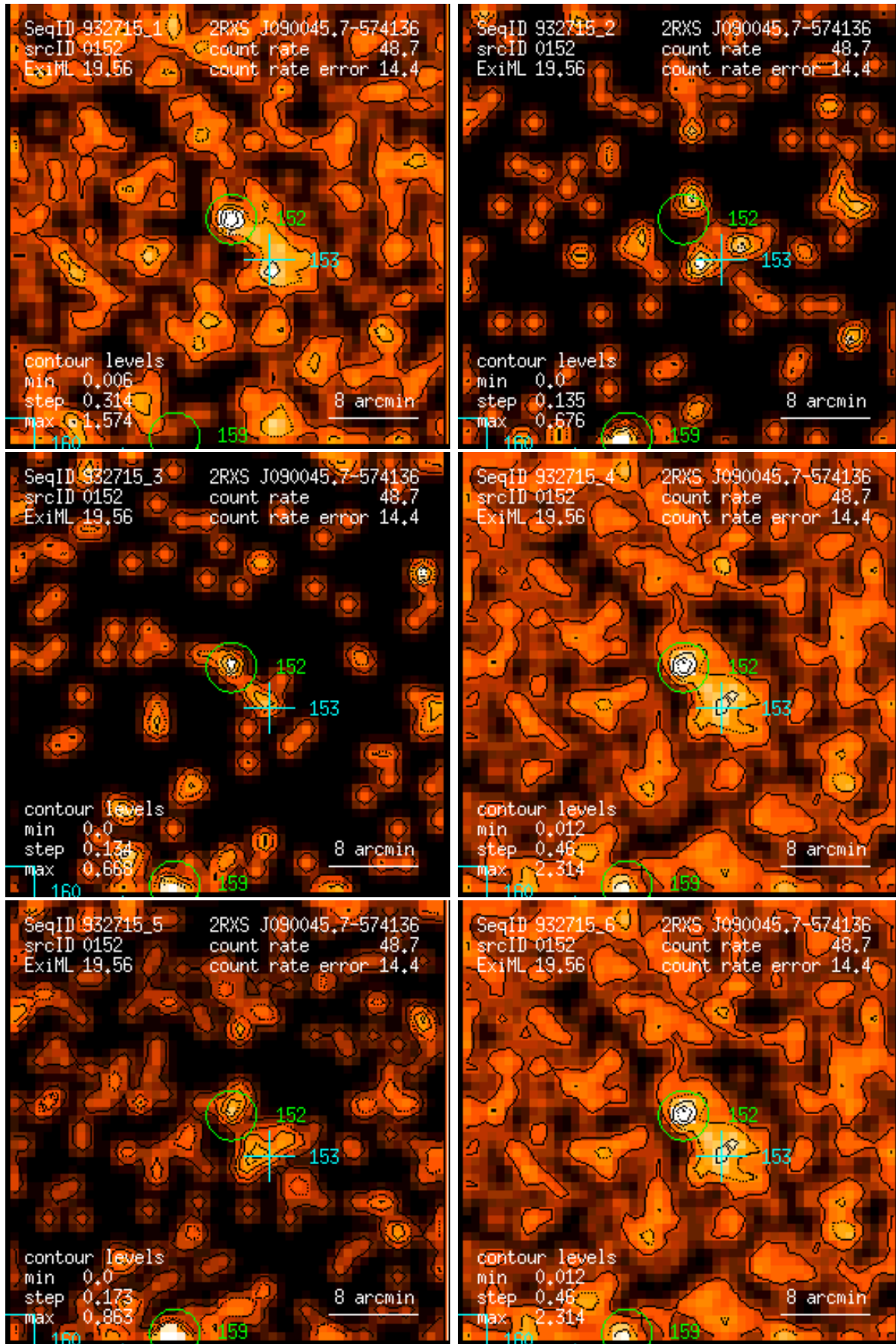
Figure 152: RASS 932715: detection 0152: band rate images, Gaussian filter: (1) PSPC channels 11 – 41, (2) 52 – 90, (3) 91 – 201, (4) 11 – 235, (5) 52 – 201, (6) 11 – 201. Broad band rates in counts/ks. Band rate contour levels in counts/ks/arcmin 2 .
