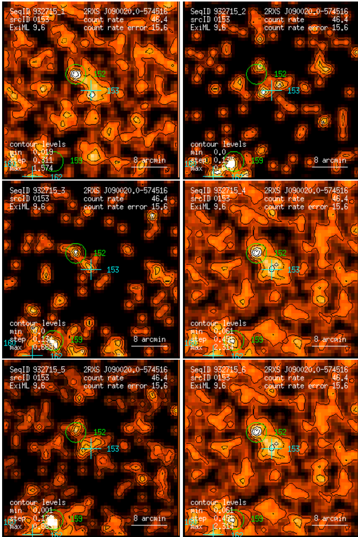
Figure 153: RASS 932715: detection 0153: band rate images, Gaussian filter: (1) PSPC channels 11 – 41, (2) 52 – 90, (3) 91 – 201, (4) 11 – 235, (5) 52 – 201, (6) 11 – 201. Broad band rates in counts/ks. Band rate contour levels in counts/ks/arcmin 2 .
