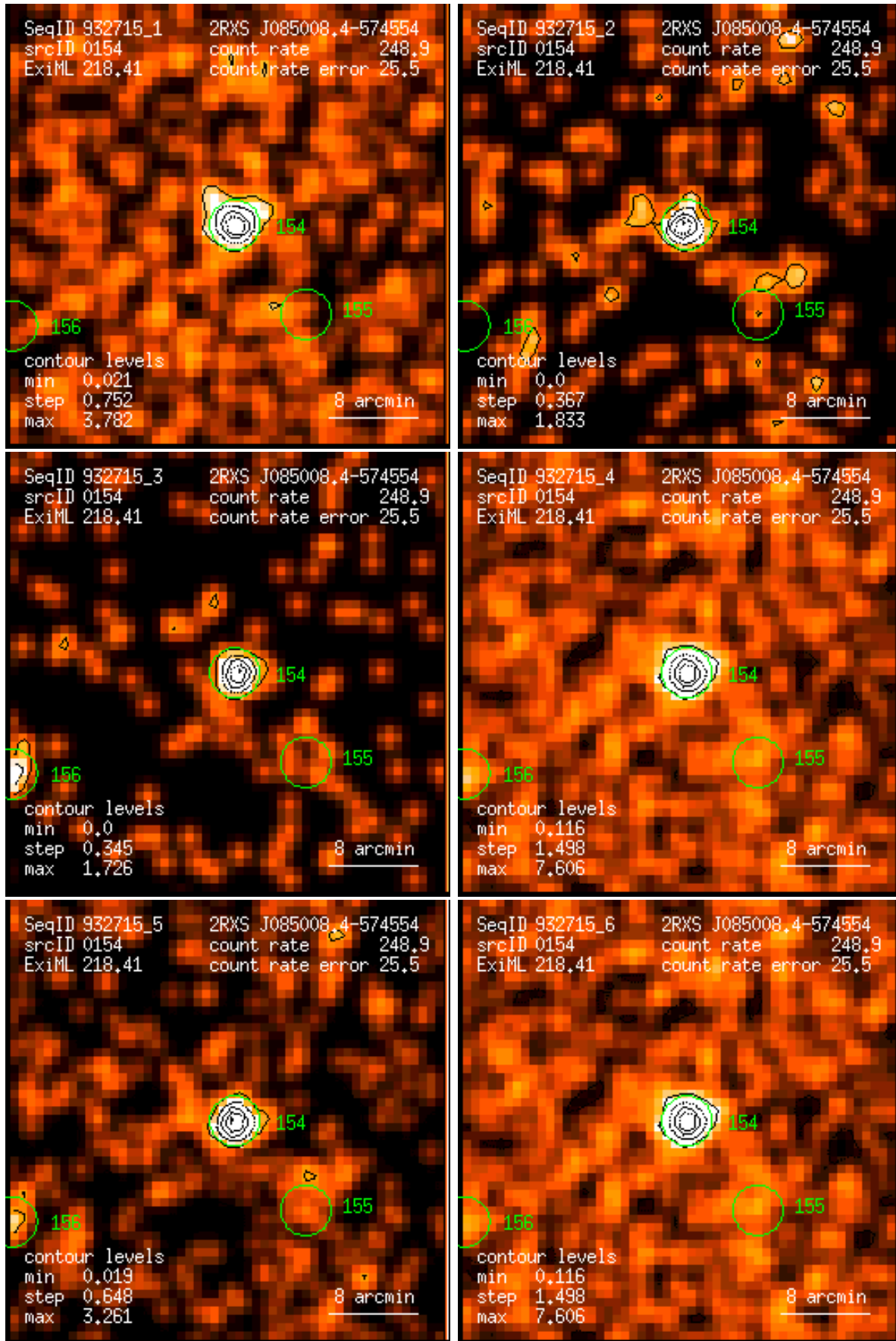
Figure 154: RASS 932715: detection 0154: band rate images, Gaussian filter: (1) PSPC channels 11 – 41, (2) 52 – 90, (3) 91 – 201, (4) 11 – 235, (5) 52 – 201, (6) 11 – 201. Broad band rates in counts/ks. Band rate contour levels in counts/ks/arcmin 2 .
