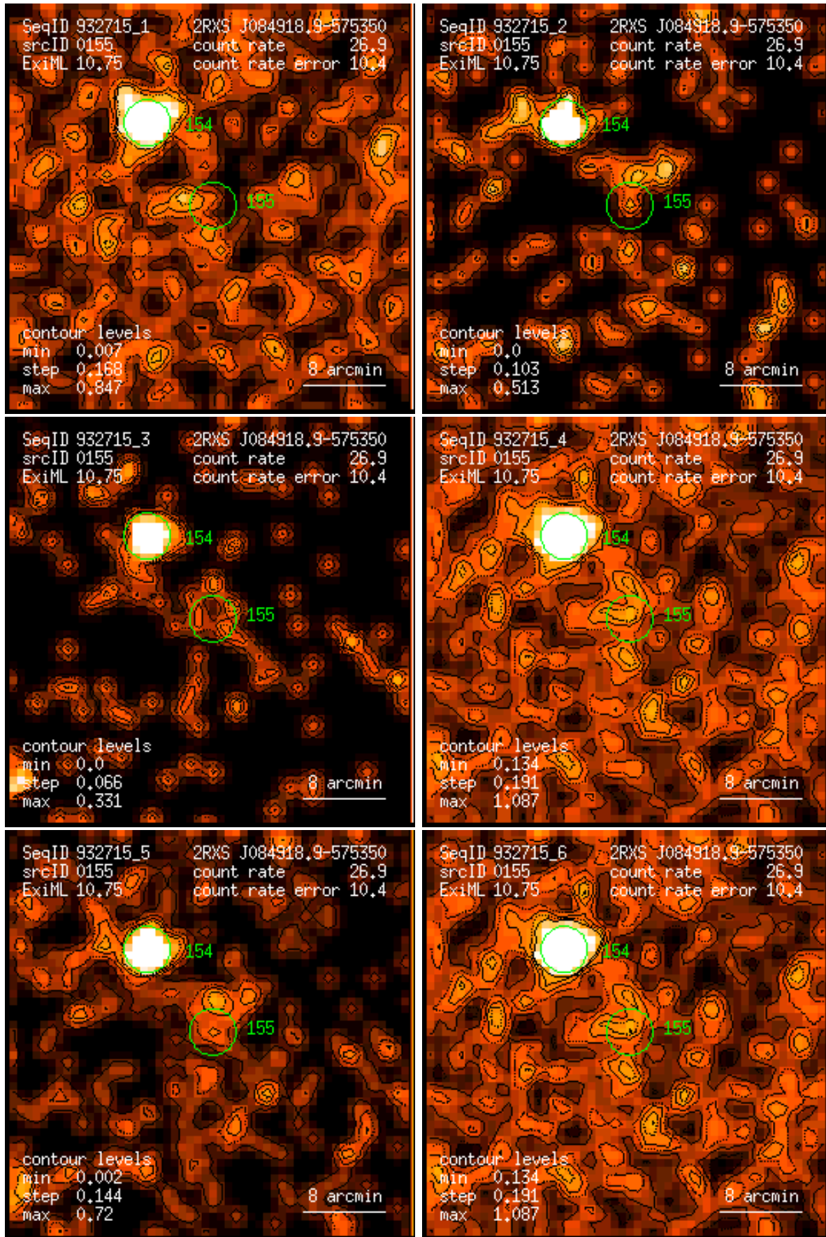
Figure 155: RASS 932715: detection 0155: band rate images, Gaussian filter: (1) PSPC channels 11 – 41, (2) 52 – 90, (3) 91 – 201, (4) 11 – 235, (5) 52 – 201, (6) 11 – 201. Broad band rates in counts/ks. Band rate contour levels in counts/ks/arcmin 2 .
