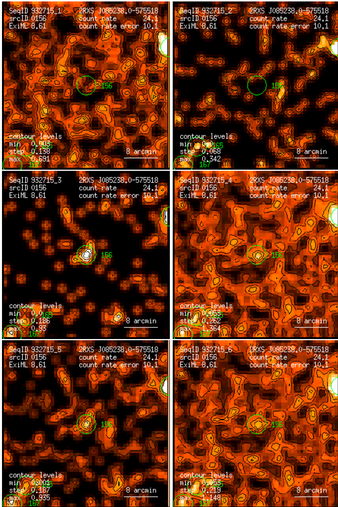
Figure 156: RASS 932715: detection 0156: band rate images, Gaussian filter: (1) PSPC channels 11 – 41, (2) 52 – 90, (3) 91 – 201, (4) 11 – 235, (5) 52 – 201, (6) 11 – 201. Broad band rates in counts/ks. Band rate contour levels in counts/ks/arcmin 2 .
