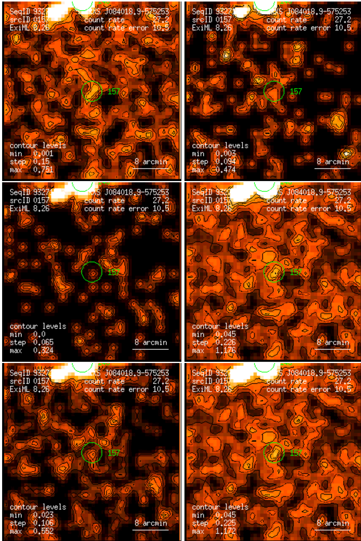
Figure 157: RASS 932715: detection 0157: band rate images, Gaussian filter: (1) PSPC channels 11 – 41, (2) 52 – 90, (3) 91 – 201, (4) 11 – 235, (5) 52 – 201, (6) 11 – 201. Broad band rates in counts/ks. Band rate contour levels in counts/ks/arcmin 2 .
