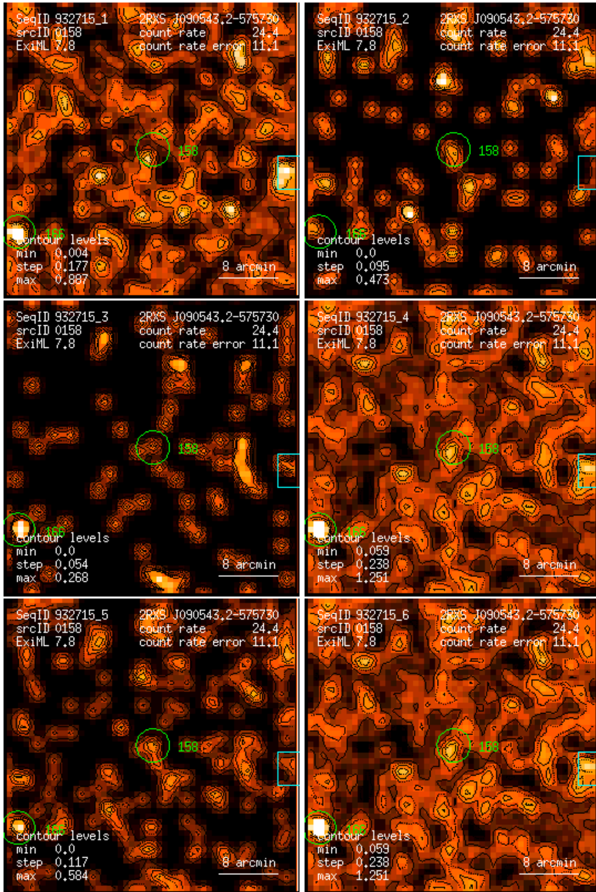
Figure 158: RASS 932715: detection 0158: band rate images, Gaussian filter: (1) PSPC channels 11 – 41, (2) 52 – 90, (3) 91 – 201, (4) 11 – 235, (5) 52 – 201, (6) 11 – 201. Broad band rates in counts/ks. Band rate contour levels in counts/ks/arcmin 2 .
