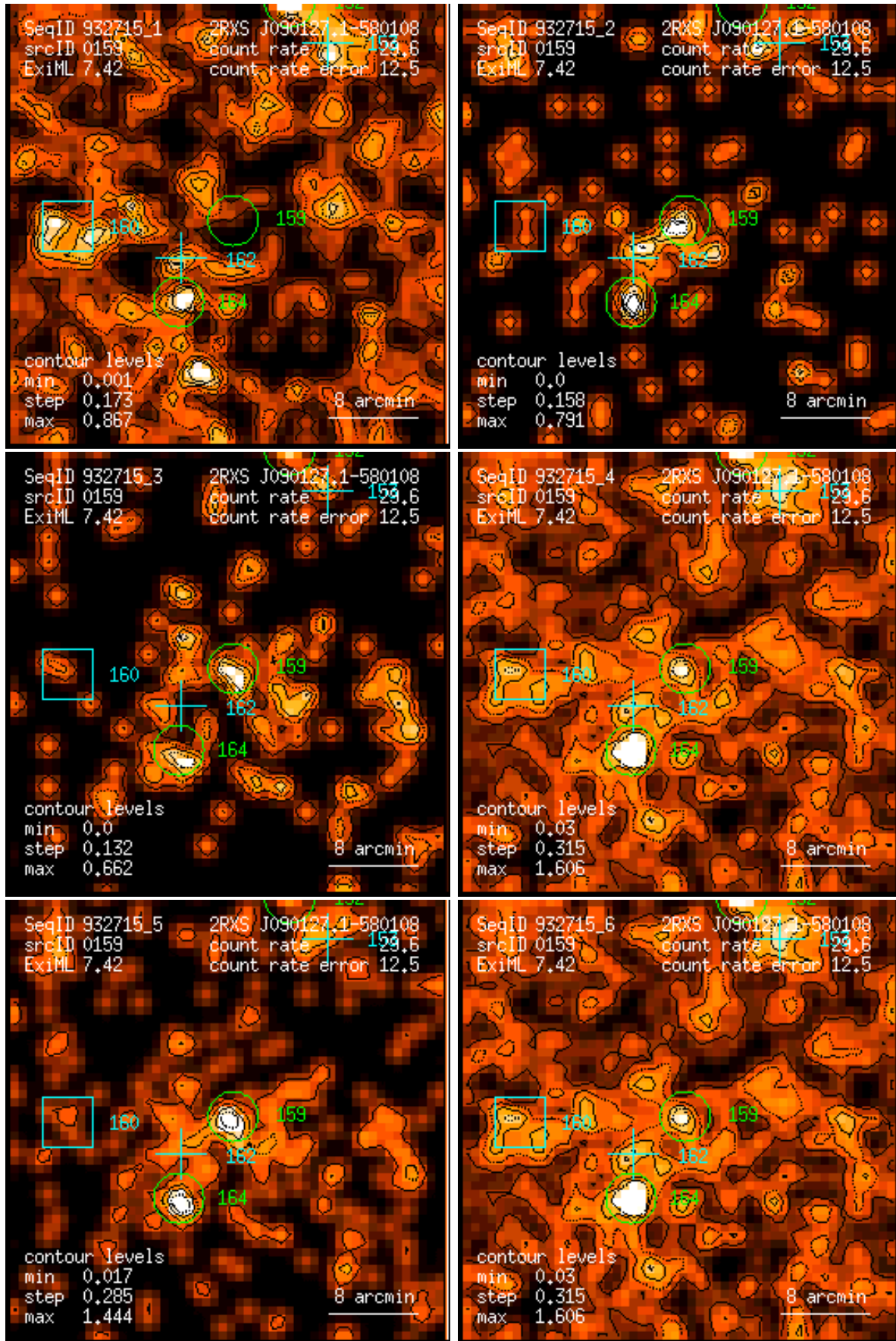
Figure 159: RASS 932715: detection 0159: band rate images, Gaussian filter: (1) PSPC channels 11 – 41, (2) 52 – 90, (3) 91 – 201, (4) 11 – 235, (5) 52 – 201, (6) 11 – 201. Broad band rates in counts/ks. Band rate contour levels in counts/ks/arcmin 2 .
