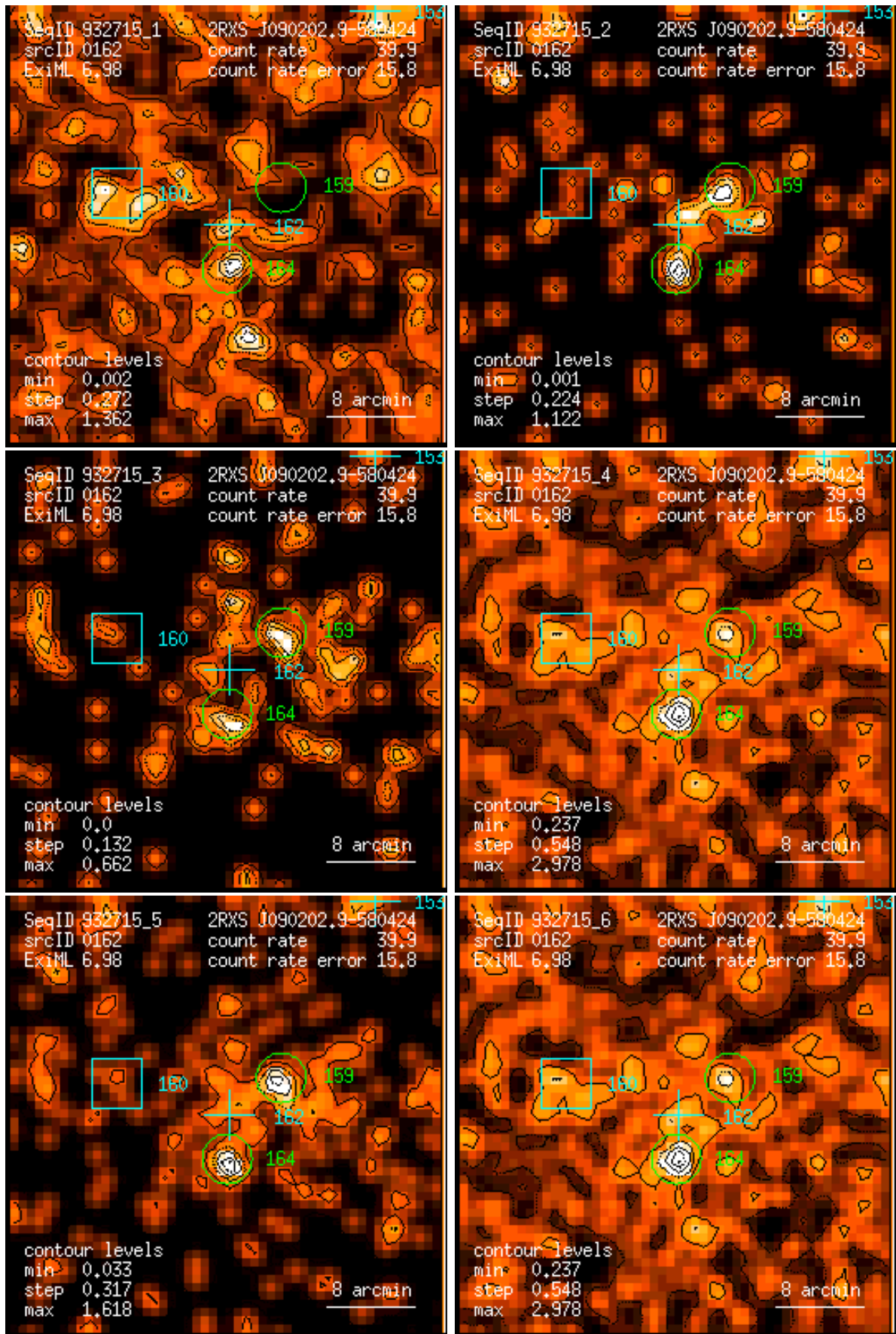
Figure 162: RASS 932715: detection 0162: band rate images, Gaussian filter: (1) PSPC channels 11 – 41, (2) 52 – 90, (3) 91 – 201, (4) 11 – 235, (5) 52 – 201, (6) 11 – 201. Broad band rates in counts/ks. Band rate contour levels in counts/ks/arcmin 2 .
