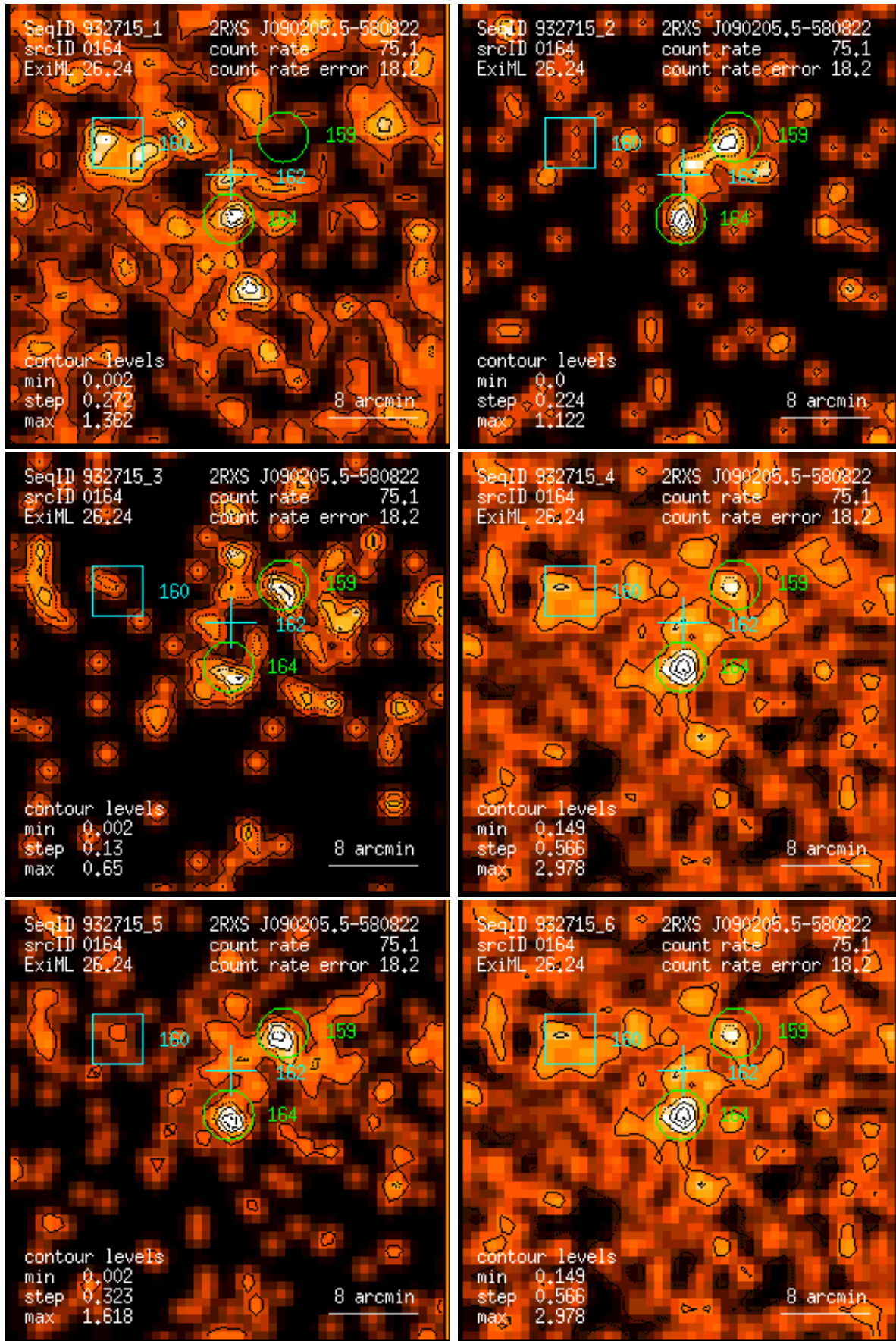
Figure 164: RASS 932715: detection 0164: band rate images, Gaussian filter: (1) PSPC channels 11 – 41, (2) 52 – 90, (3) 91 – 201, (4) 11 – 235, (5) 52 – 201, (6) 11 – 201. Broad band rates in counts/ks. Band rate contour levels in counts/ks/arcmin 2 .
