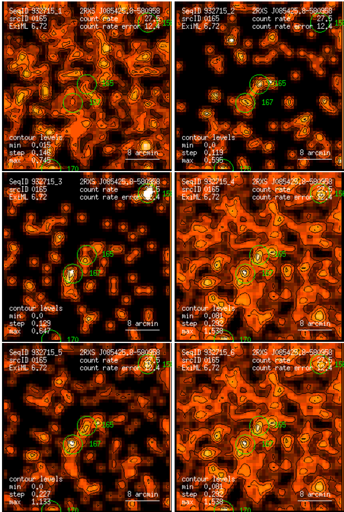
Figure 165: RASS 932715: detection 0165: band rate images, Gaussian filter: (1) PSPC channels 11 – 41, (2) 52 – 90, (3) 91 – 201, (4) 11 – 235, (5) 52 – 201, (6) 11 – 201. Broad band rates in counts/ks. Band rate contour levels in counts/ks/arcmin 2 .
