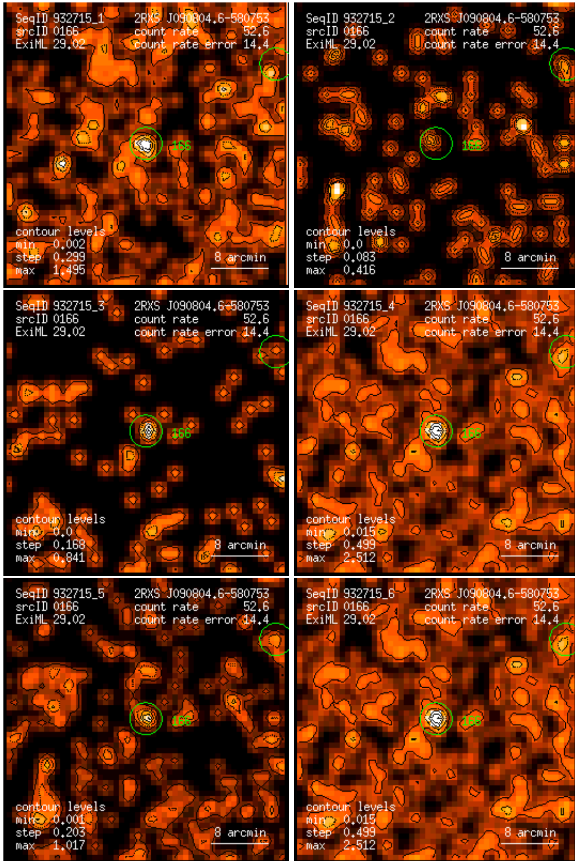
Figure 166: RASS 932715: detection 0166: band rate images, Gaussian filter: (1) PSPC channels 11 – 41, (2) 52 – 90, (3) 91 – 201, (4) 11 – 235, (5) 52 – 201, (6) 11 – 201. Broad band rates in counts/ks. Band rate contour levels in counts/ks/arcmin 2 .
