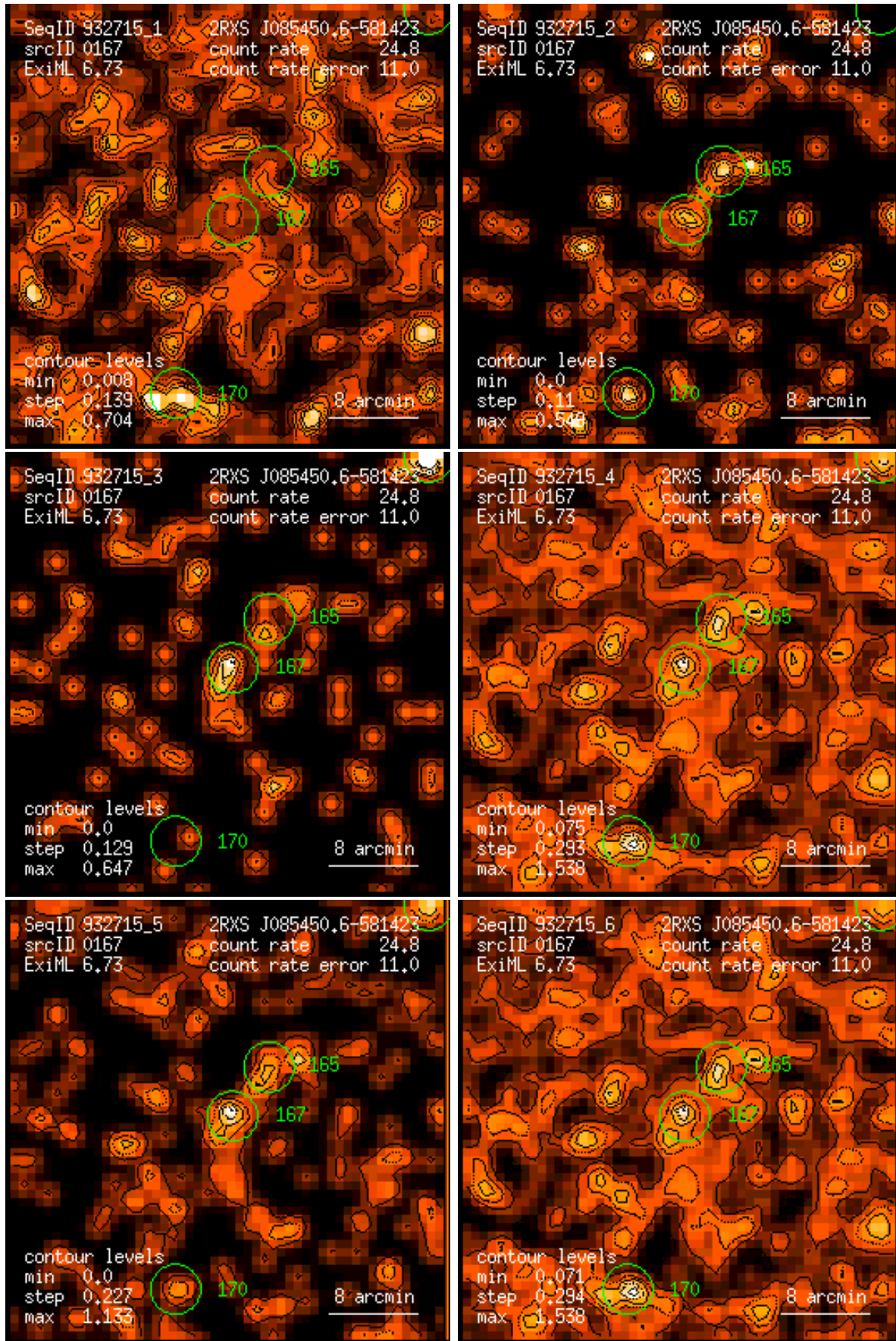
Figure 167: RASS 932715: detection 0167: band rate images, Gaussian filter: (1) PSPC channels 11 – 41, (2) 52 – 90, (3) 91 – 201, (4) 11 – 235, (5) 52 – 201, (6) 11 – 201. Broad band rates in counts/ks. Band rate contour levels in counts/ks/arcmin 2 .
