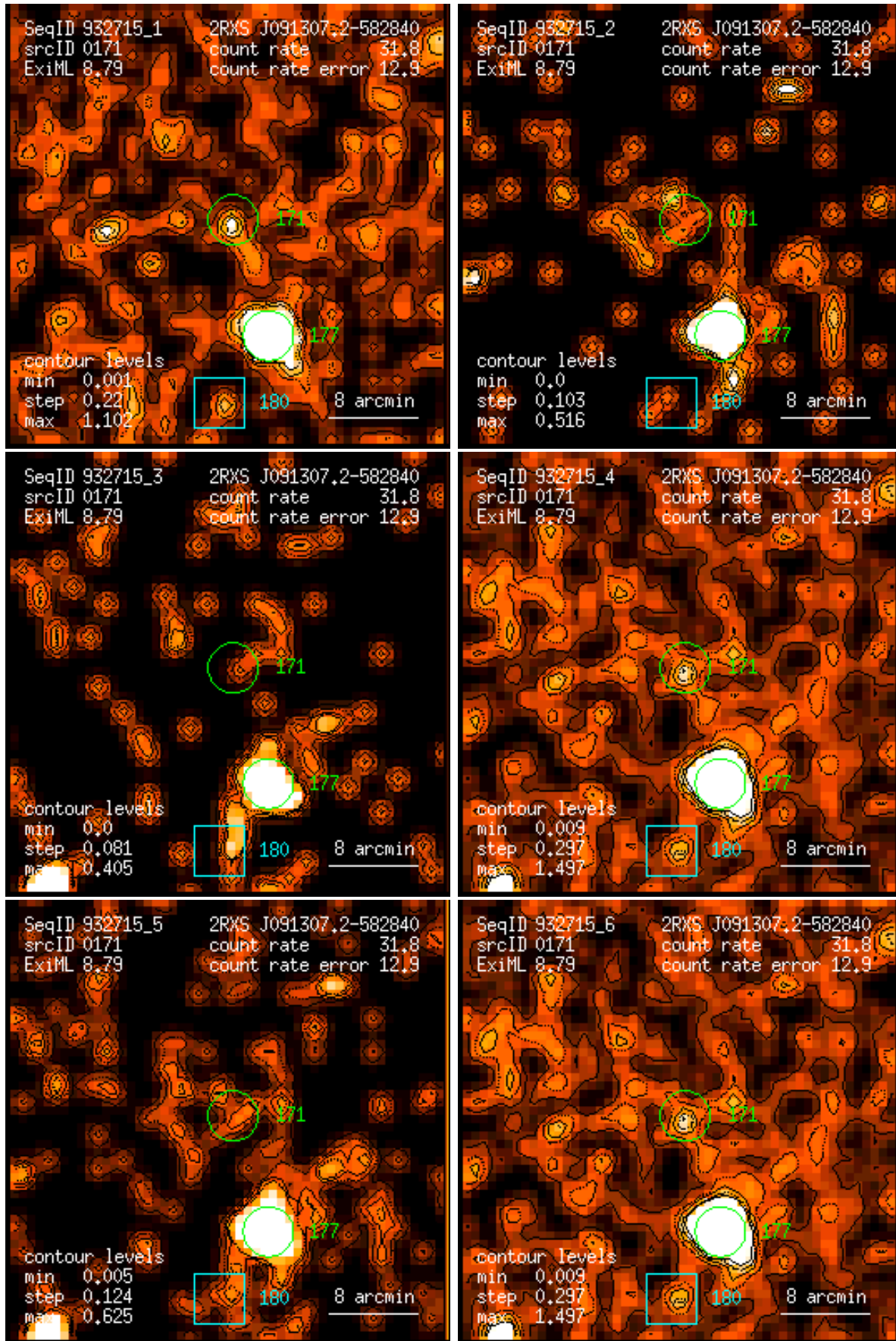
Figure 171: RASS 932715: detection 0171: band rate images, Gaussian filter: (1) PSPC channels 11 – 41, (2) 52 – 90, (3) 91 – 201, (4) 11 – 235, (5) 52 – 201, (6) 11 – 201. Broad band rates in counts/ks. Band rate contour levels in counts/ks/arcmin 2 .
